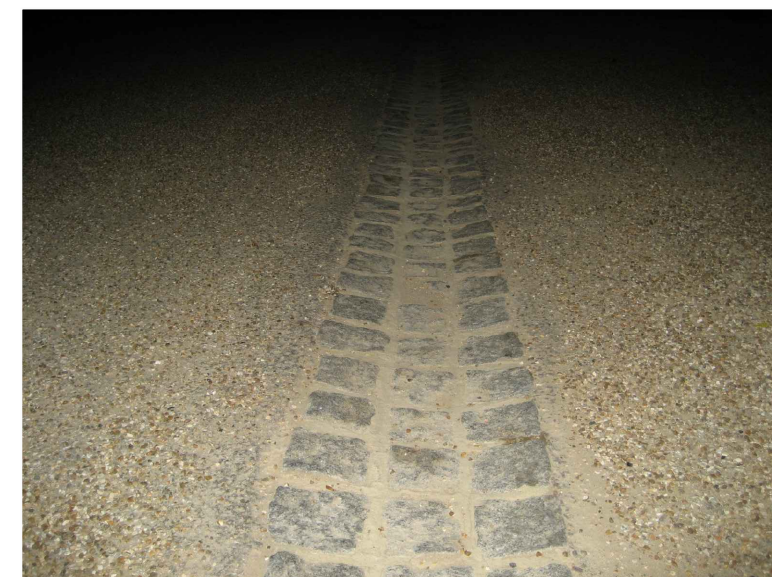
Marshalls "Conservation" Granite setts as drainage channel
