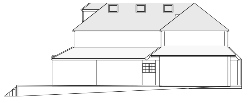
PROPOSED LEFT ELEVATION
