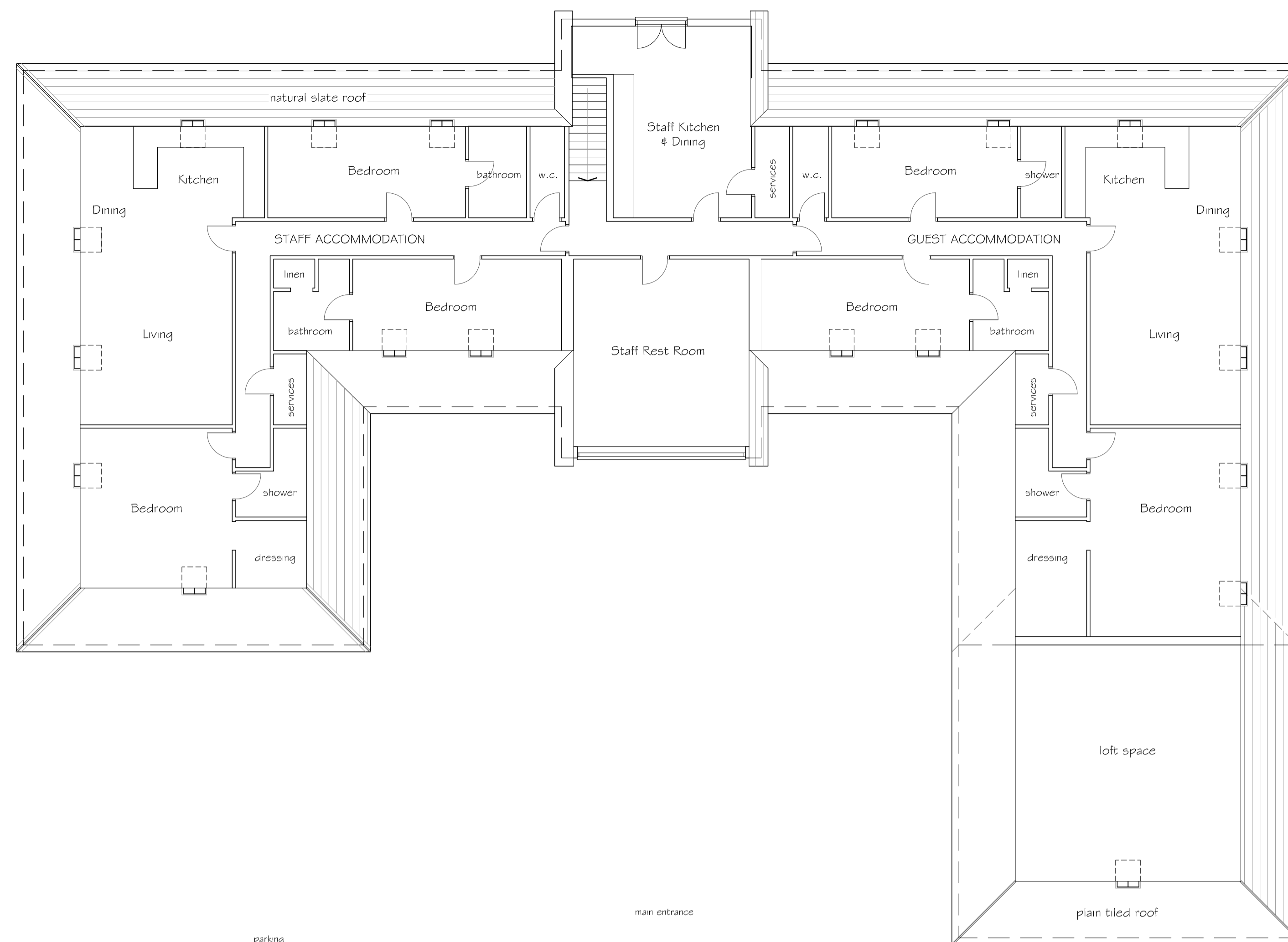
First Floor Layout
