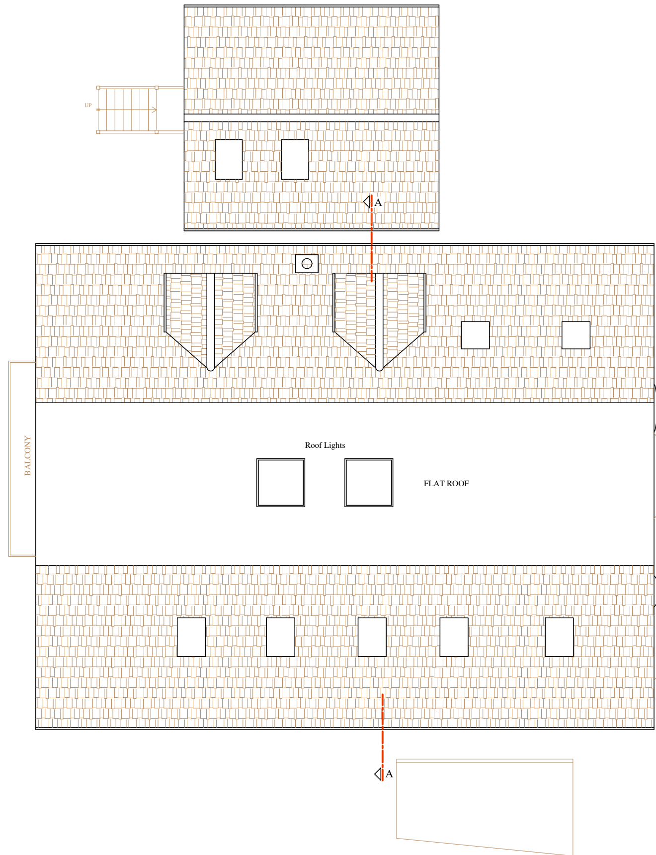
ROOF PLAN
