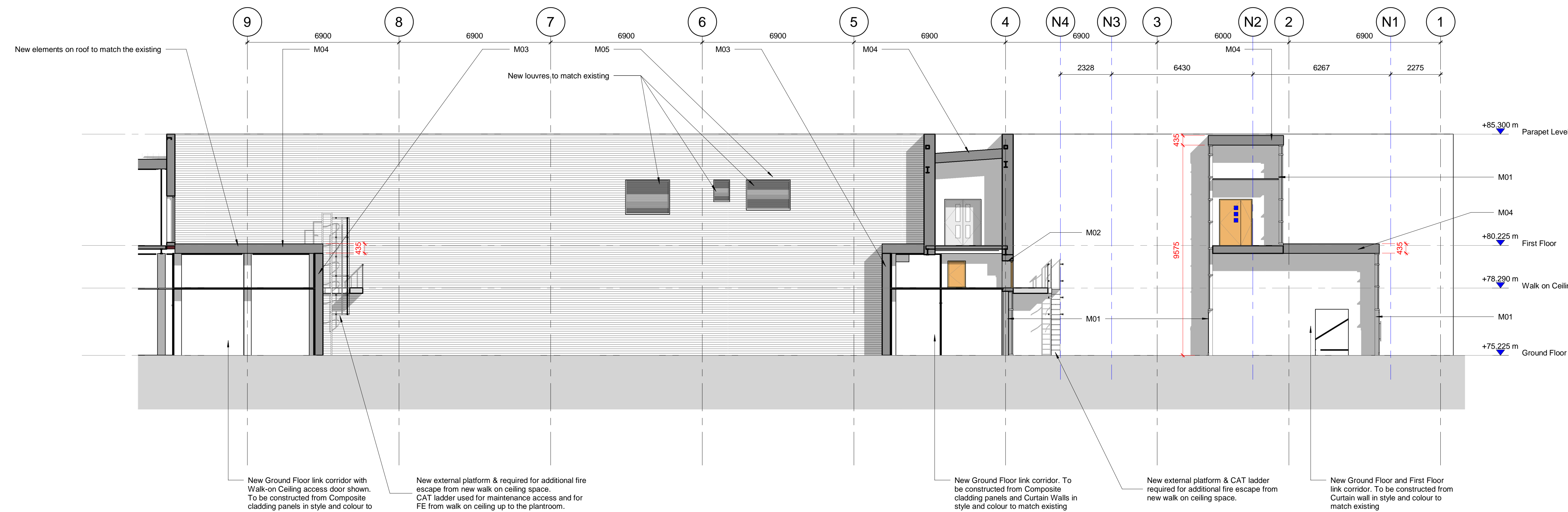
Proposed Lightwell 2 SCALE: 1:100
