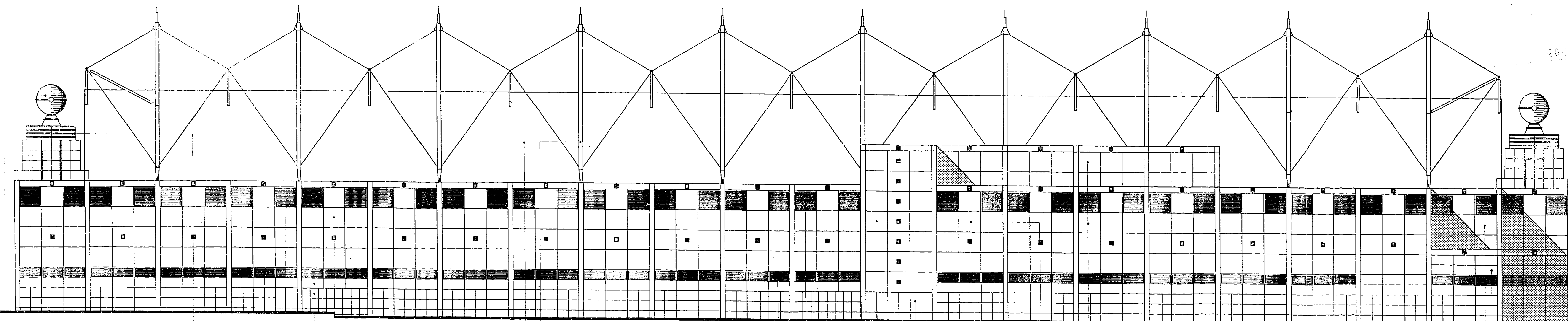
GALLERIA EAST ELEVATION
