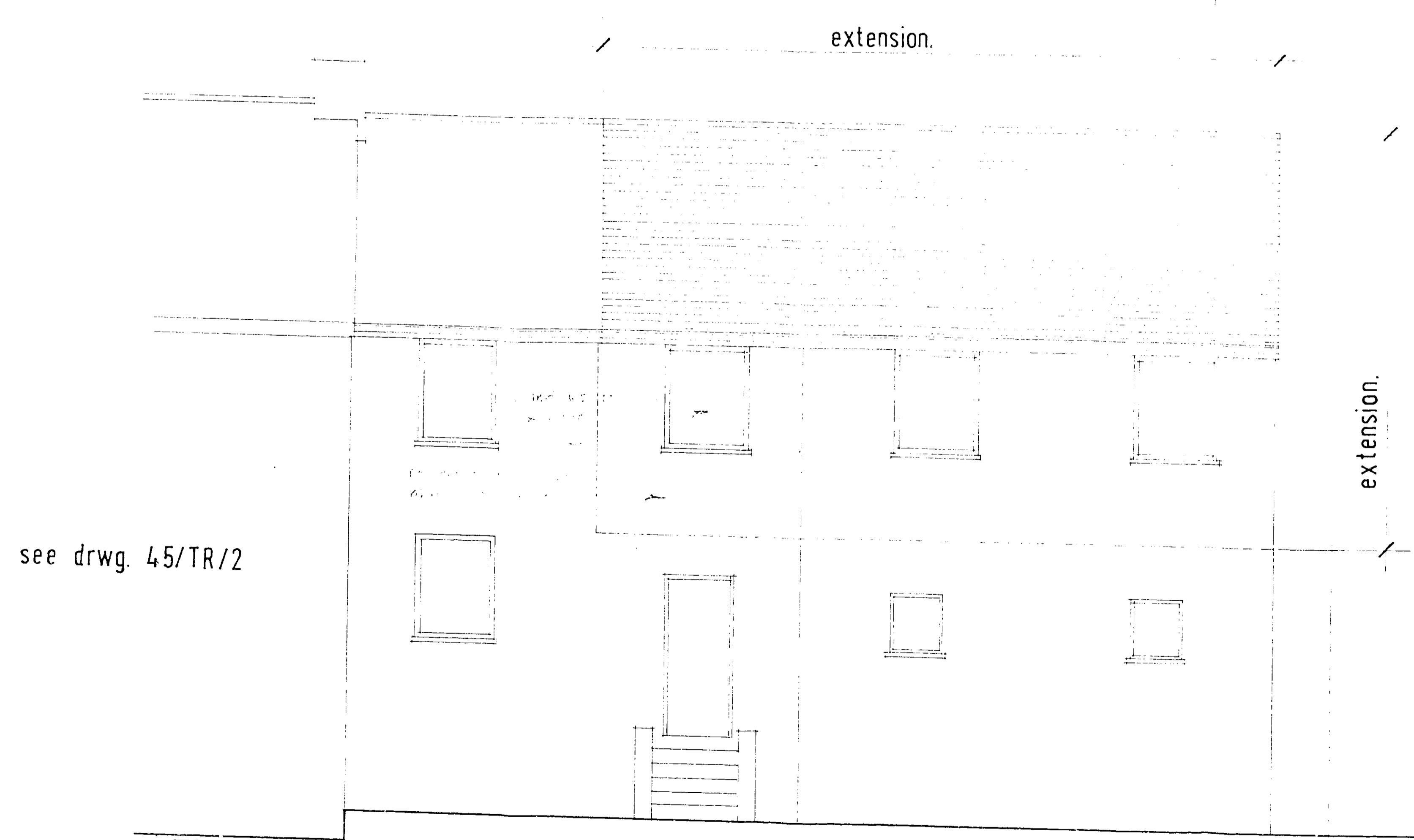
PART REAR ELEVATION AS PROPOSED.
