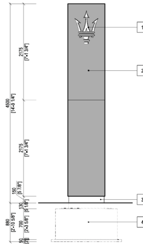
SMALL TOTEM - FRONT ELEVATION
