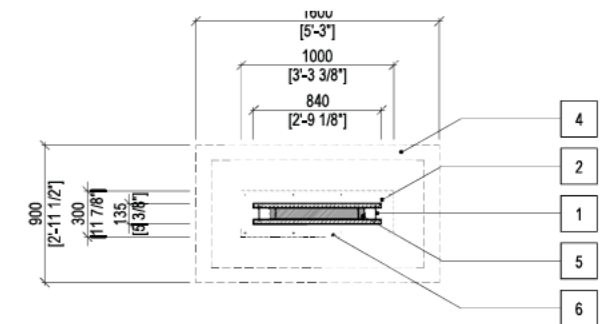
SMALL TOTEM - HORIZONTAL SECTION
