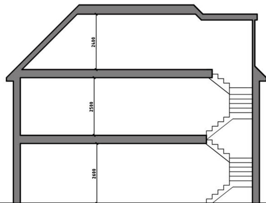
SECTION
