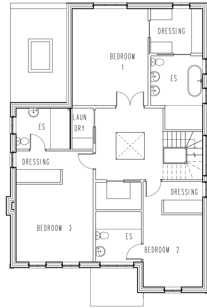
FIRST FLOOR PLAN 124M2 (EXC VOID)
