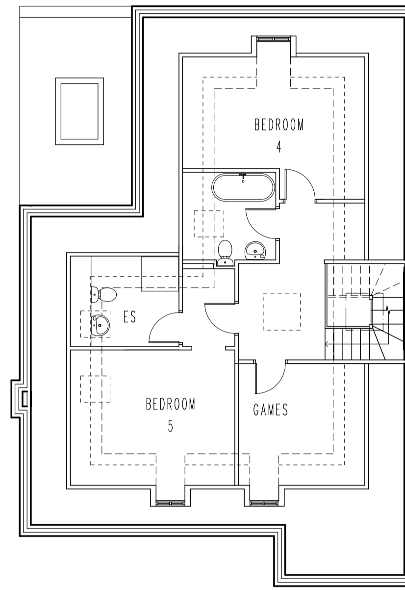
SECOND FLOOR PLAN 58M2 @ 1.5M HIGH
