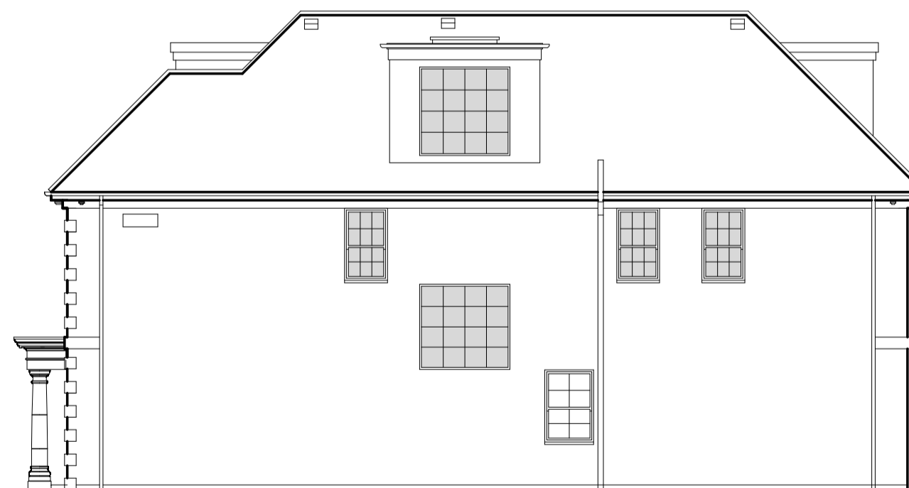
SIDE ELEVATION
