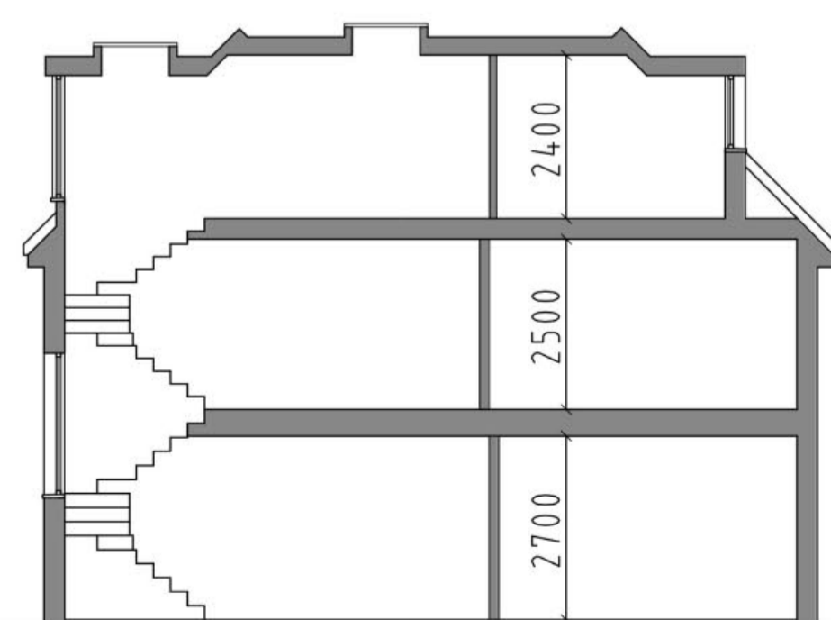
SHORT SECTION
