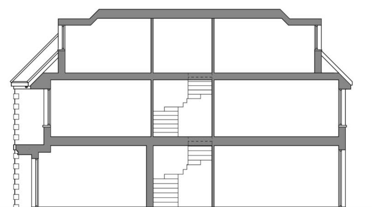
LONG SECTION
