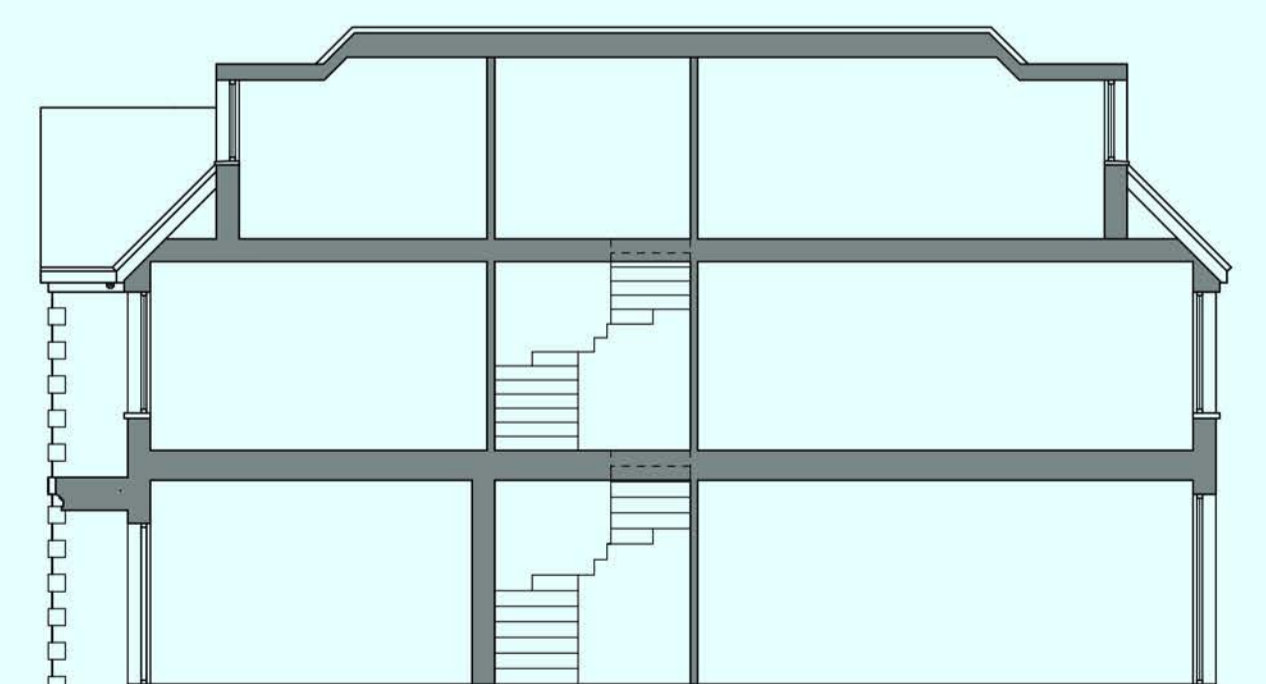
LONG SECTION
