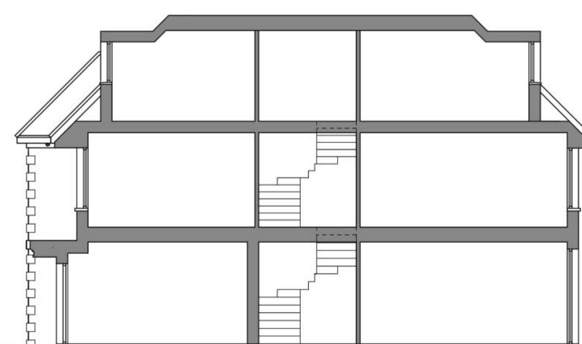
LONG SECTION
