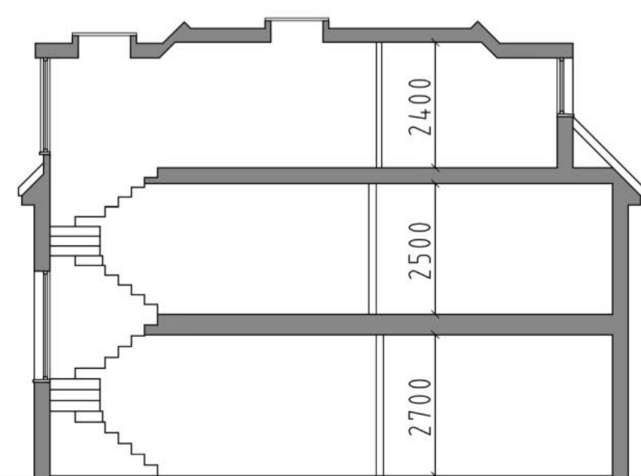
SHORT SECTION
