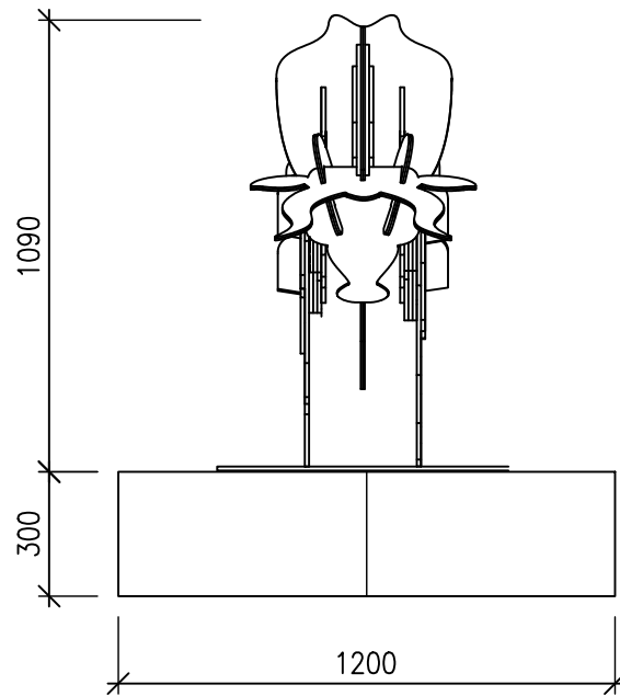
Rear Elevation
