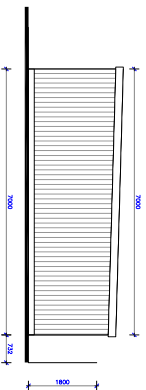
PROPOSED FLANK ELEVATION
