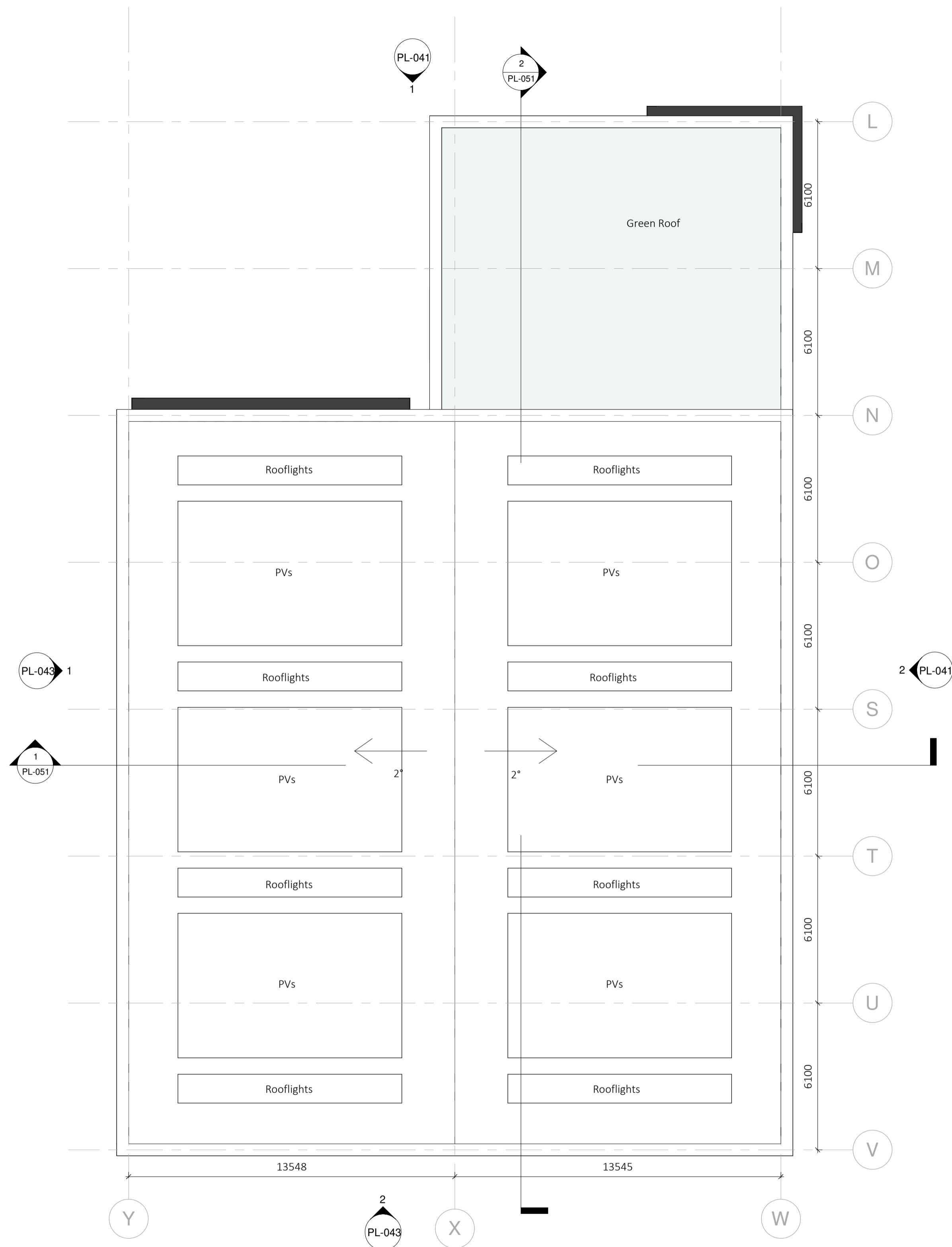
1 - Building B Roof Plan 1 : 125
