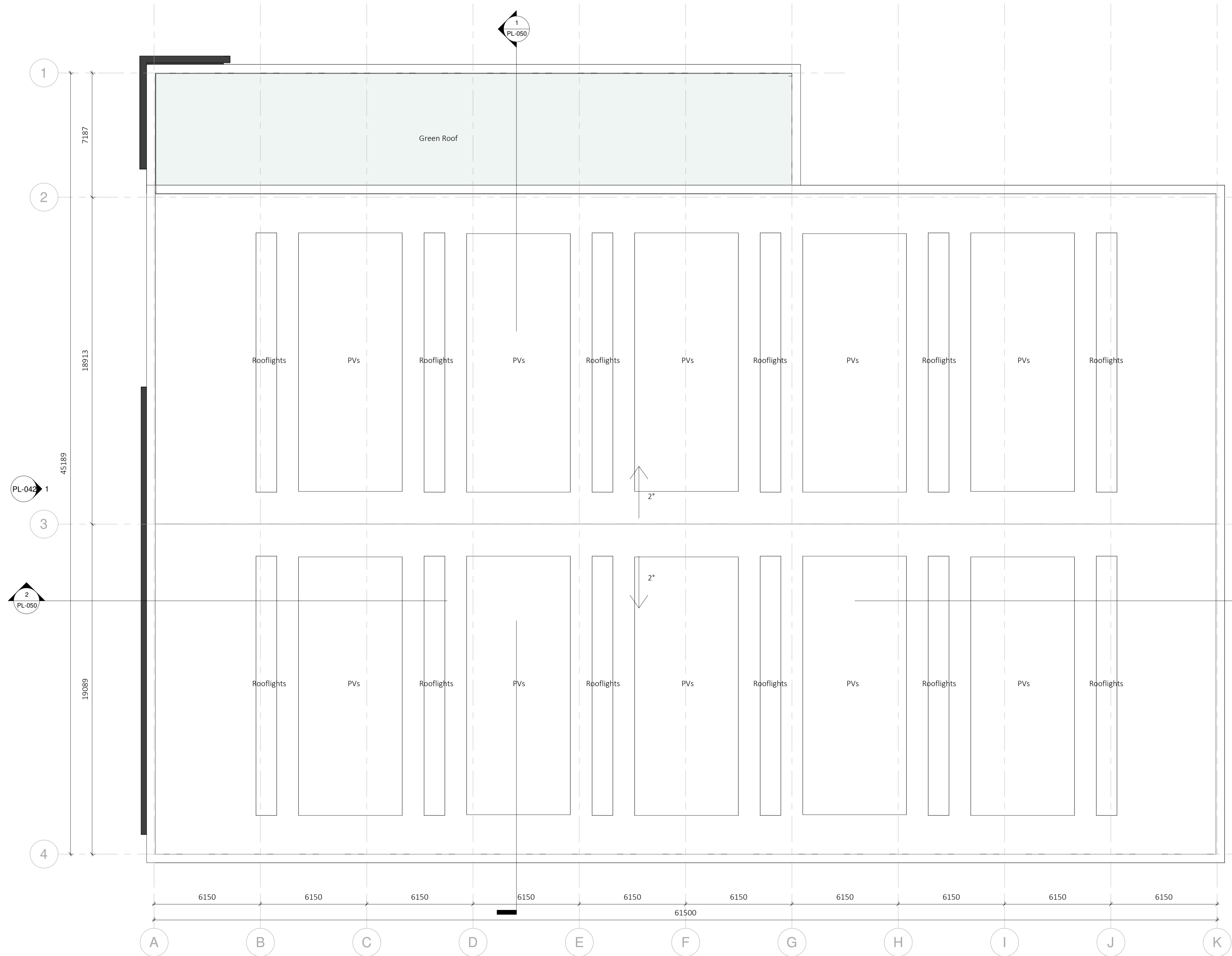
1 - Building A - Roof Plan 1:125
