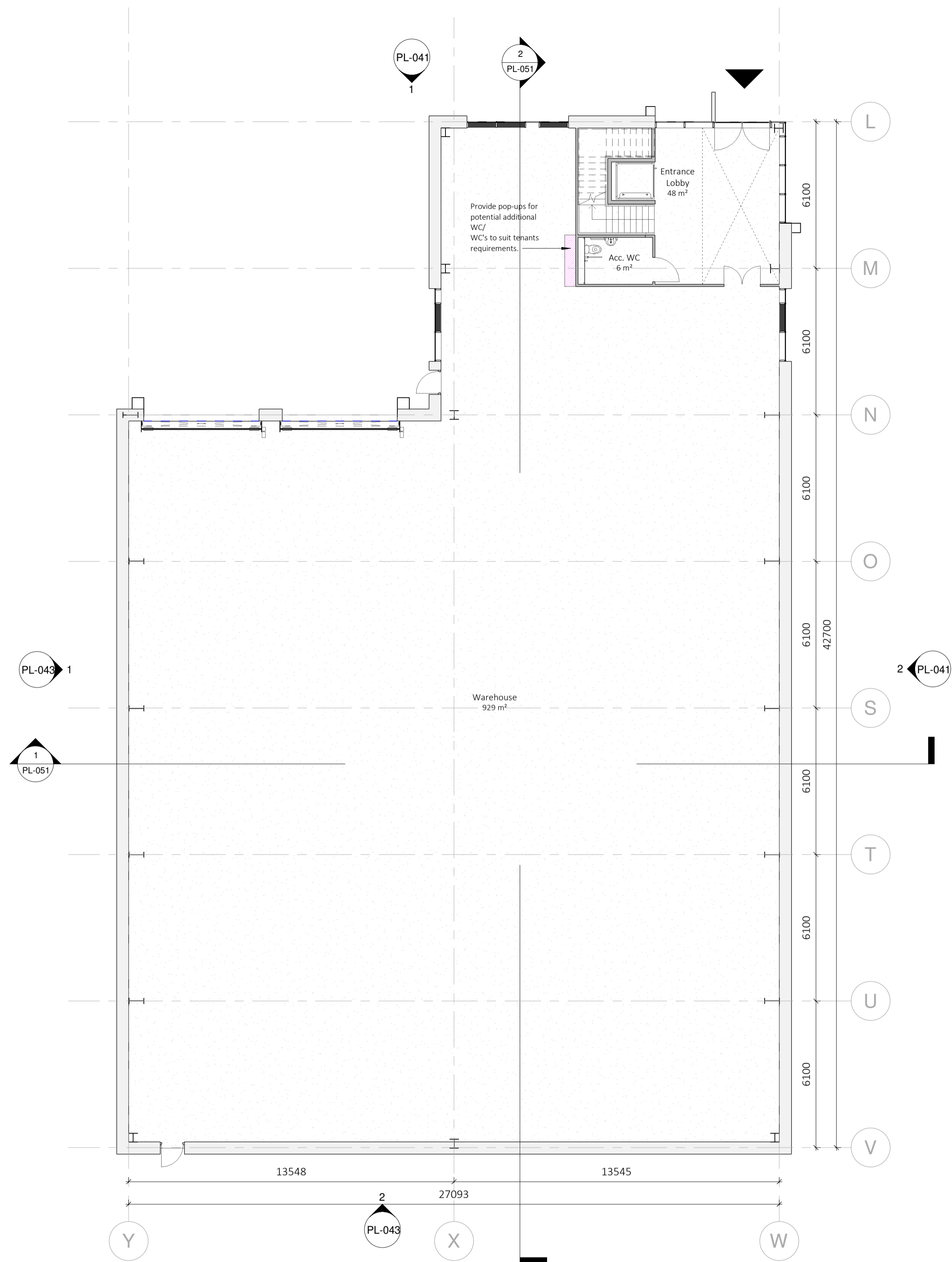
1 - Building B - Ground Floor Plan 1: 125
