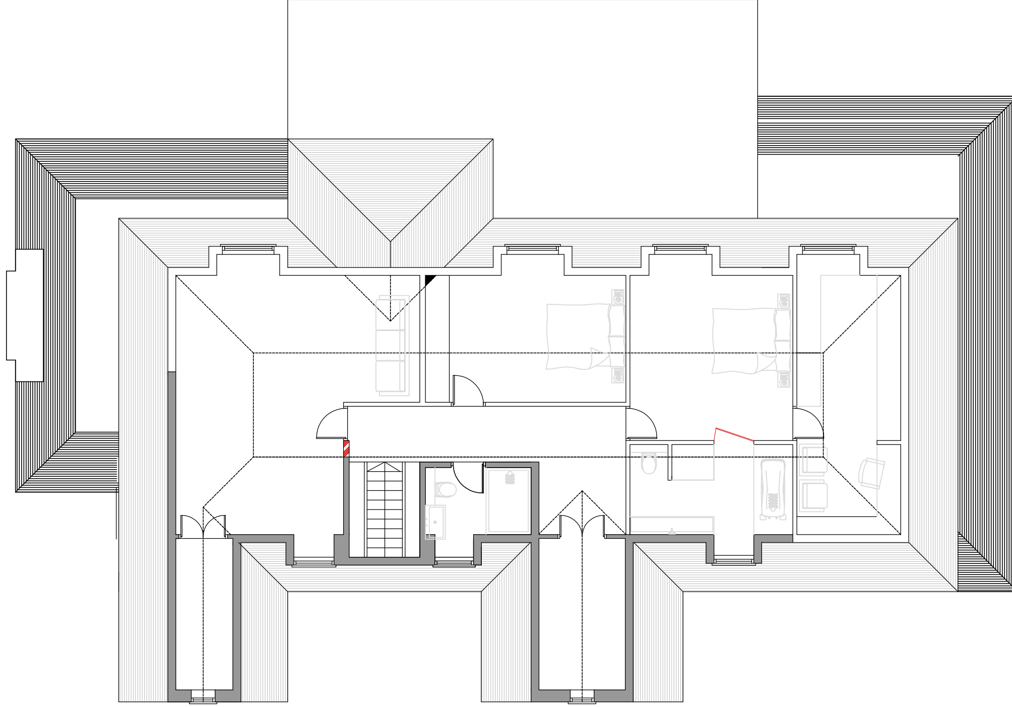
Loft Floor Plan
