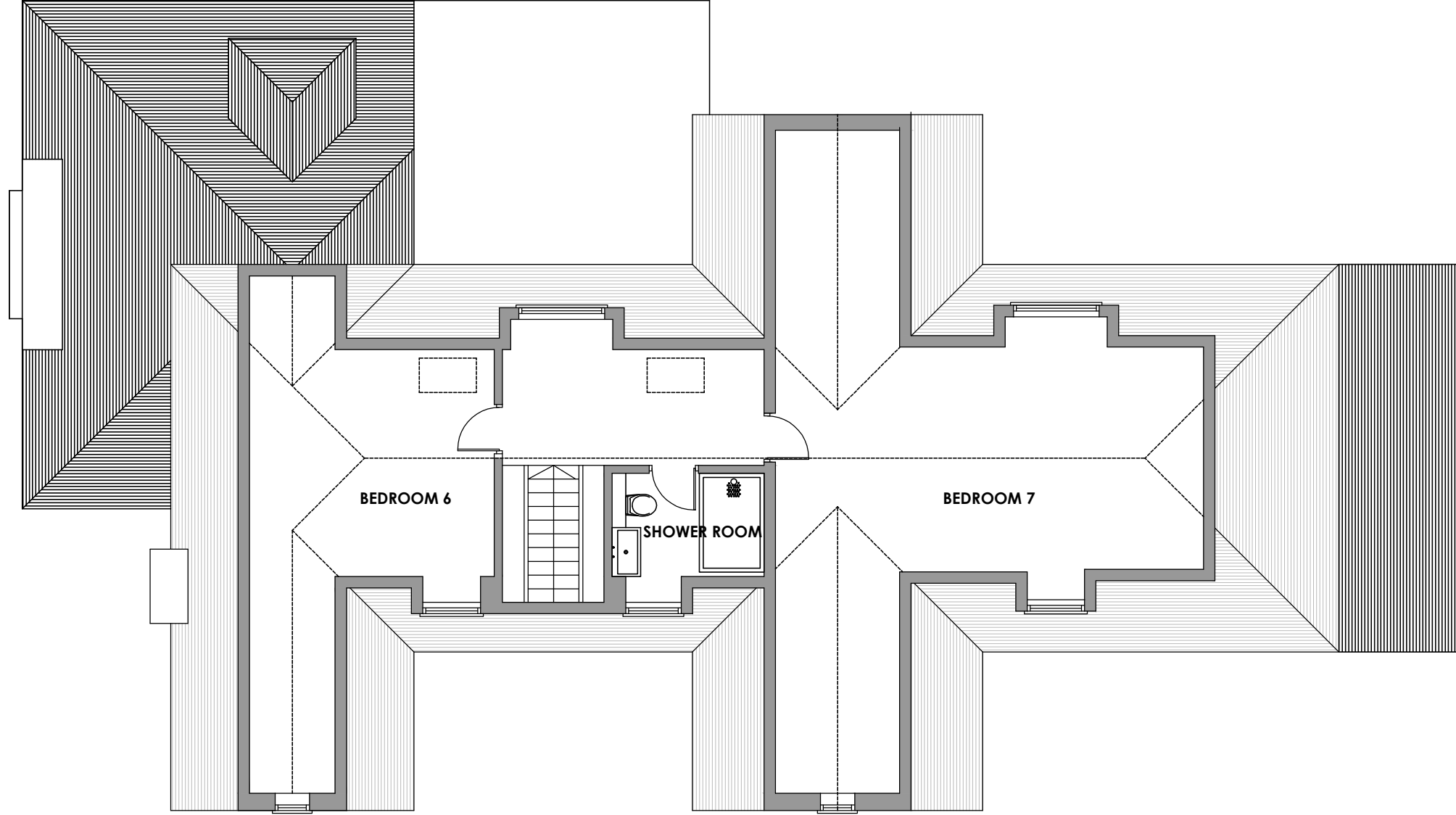
Loft Floor Plan
