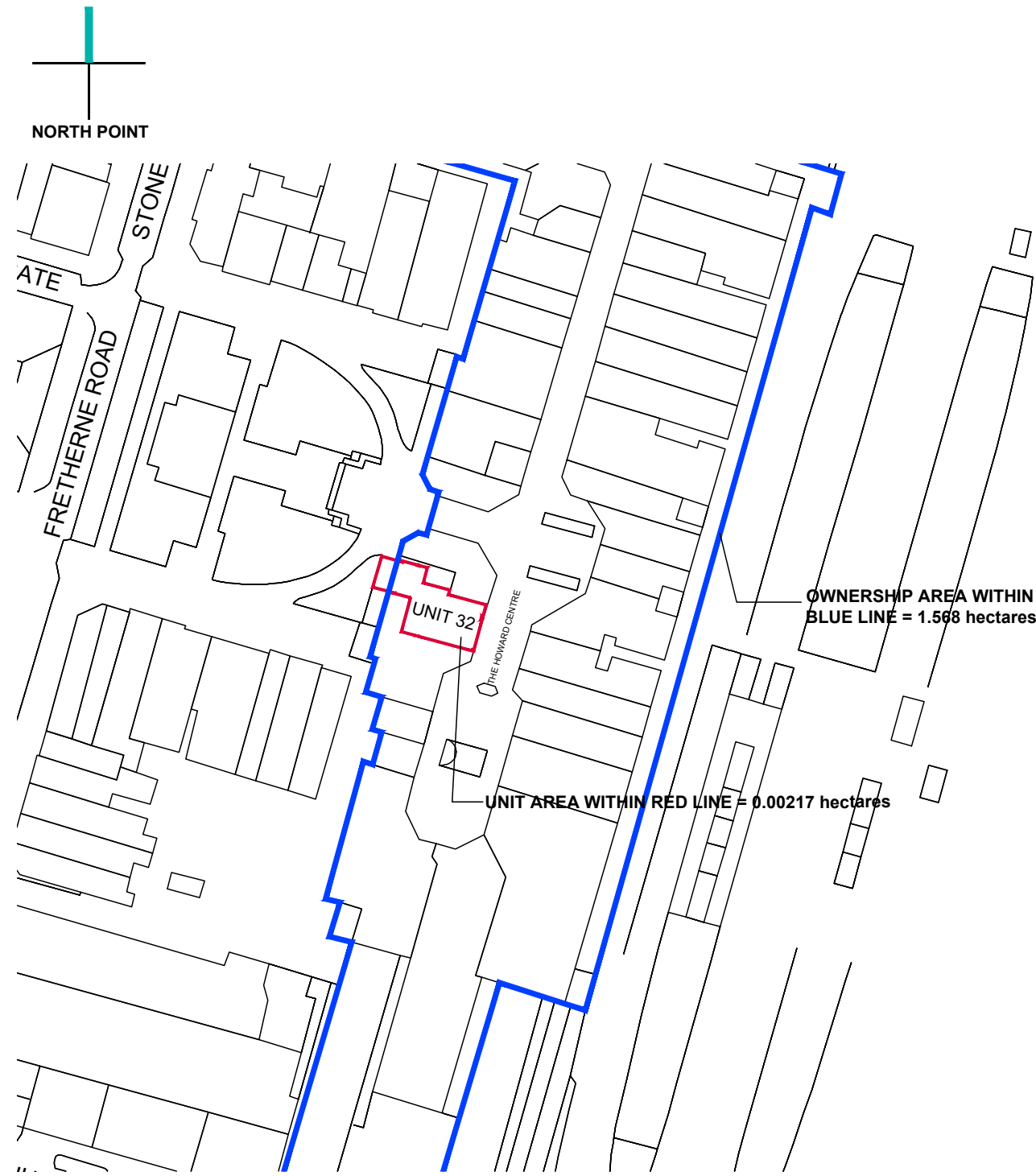
Site Location Plan SCALE 1:1250 0m 10m 25m 50m
