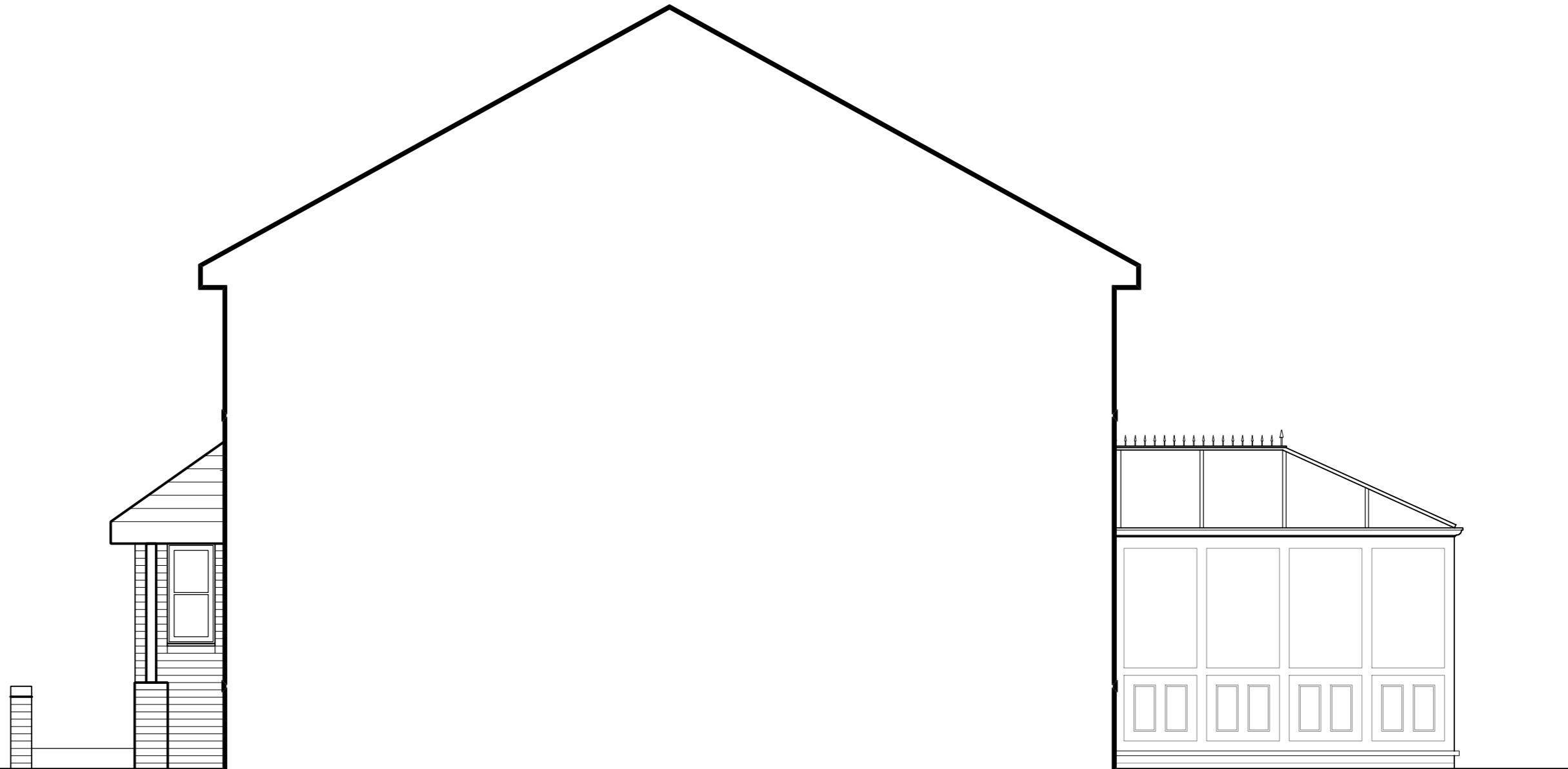
SIDE ELEVATION 1:50
