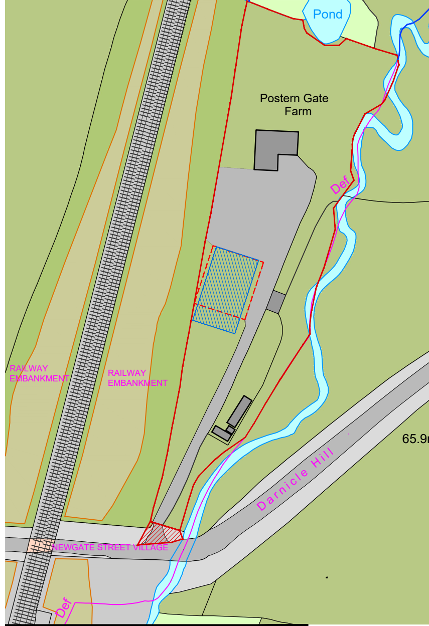
[01] LOCATION PLAN 1:1250
