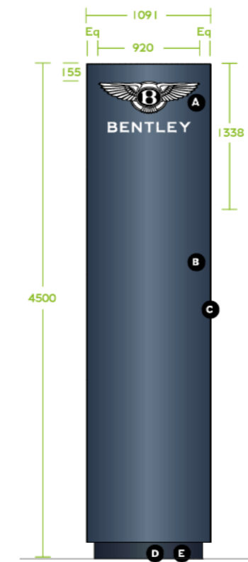
Elevation: Medium Pylon 1:50
