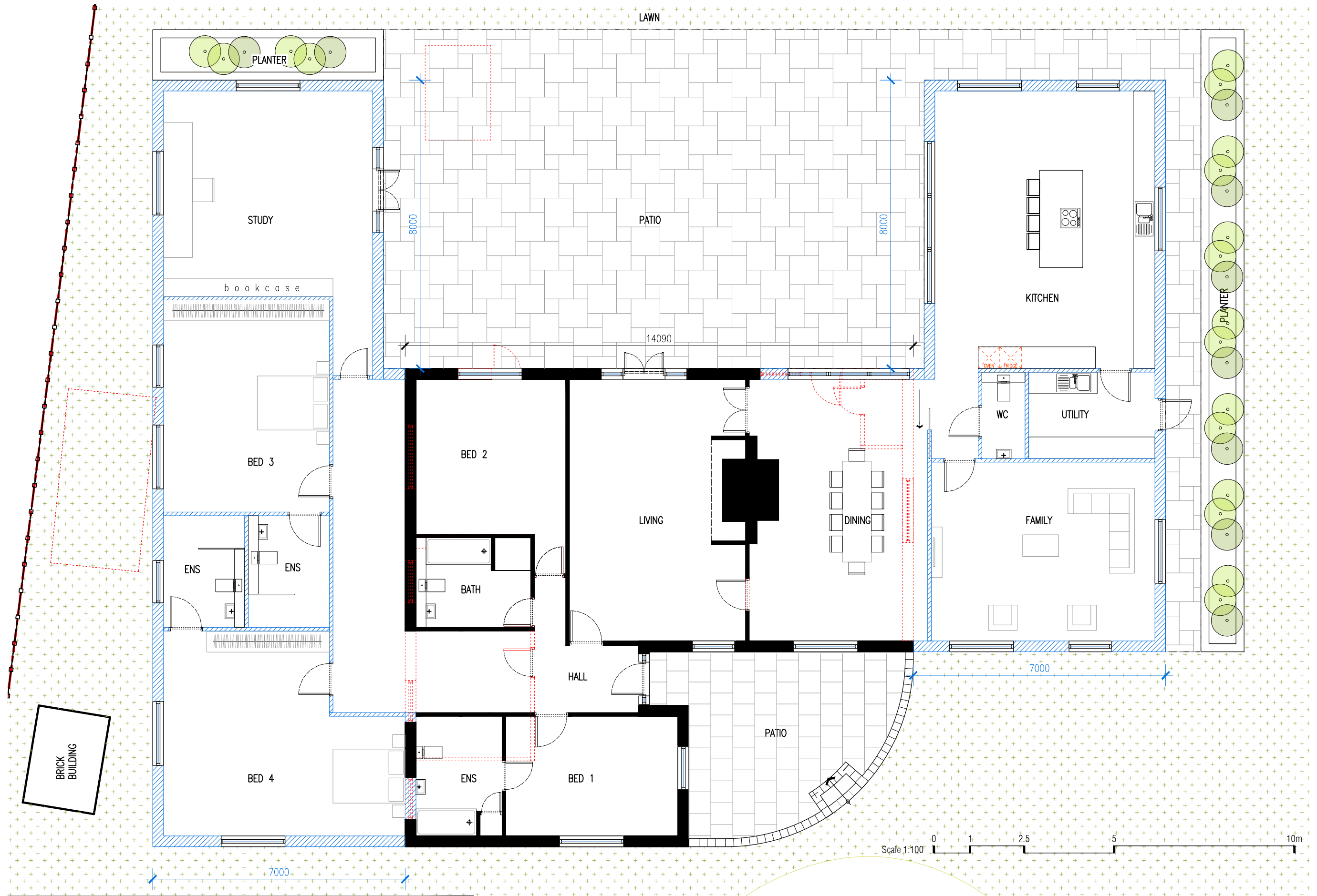
[01] PROPOSED GROUND FLOOR
