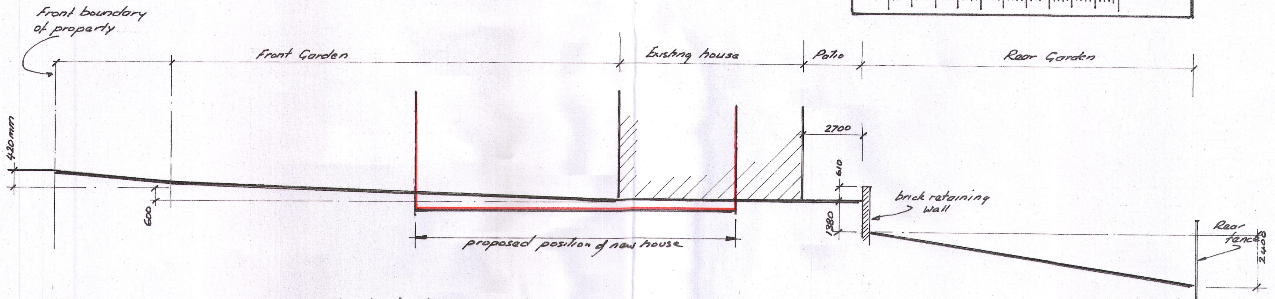
Section thro' Existing site with existing house Position 1:100 and Proposed Position of New house.
