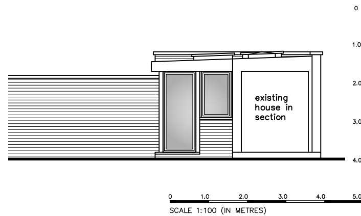
SIDE (SW) ELEVATION / SECTION
