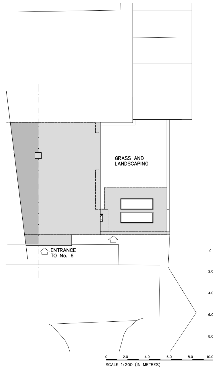
PROPOSED SITE AND ROOF PLAN 1:200
