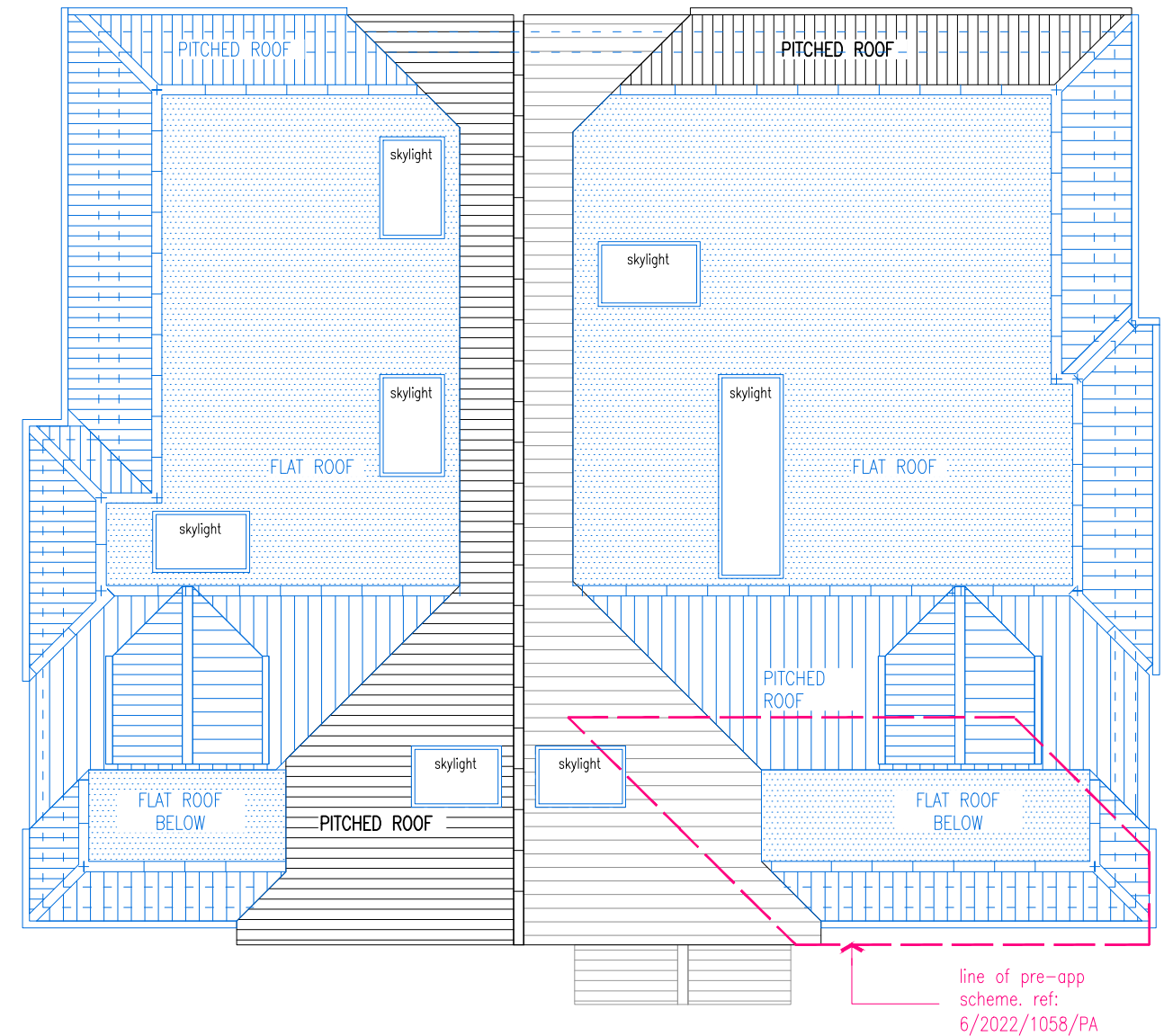
[02] PROPOSED ROOF PLAN
