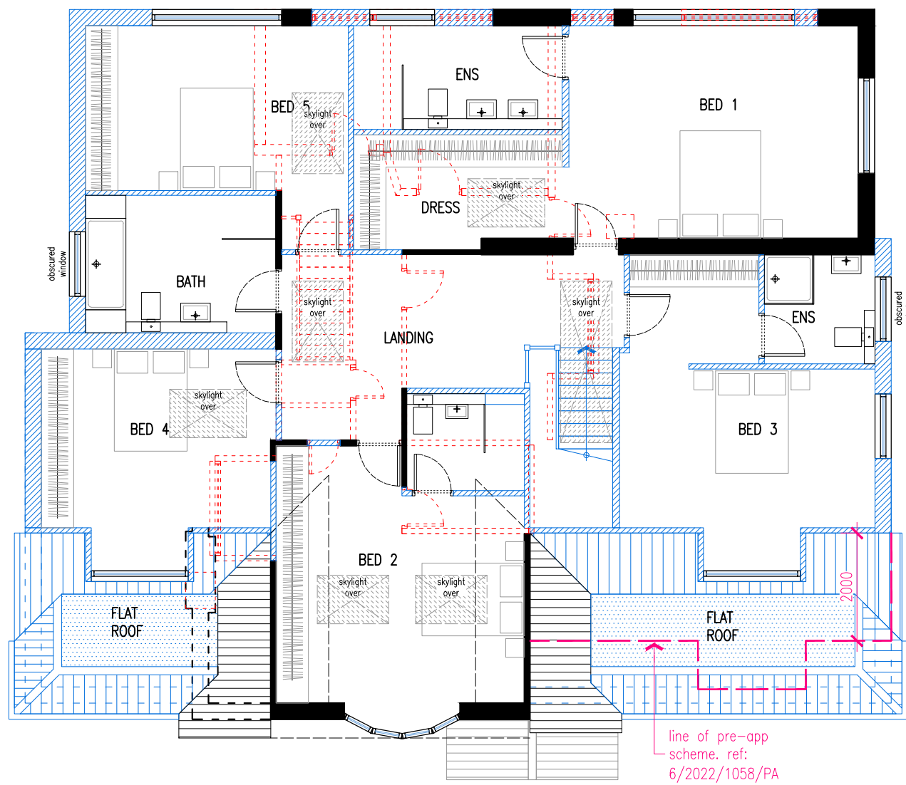
[01] PROPOSED FIRST FLOOR
