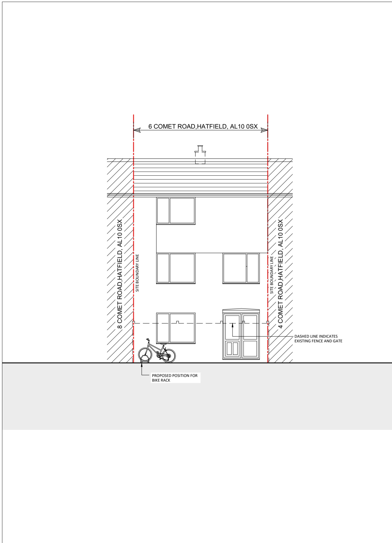
PROPOSED FRONT ELEVATION. SCALE 1:100 @ A3
