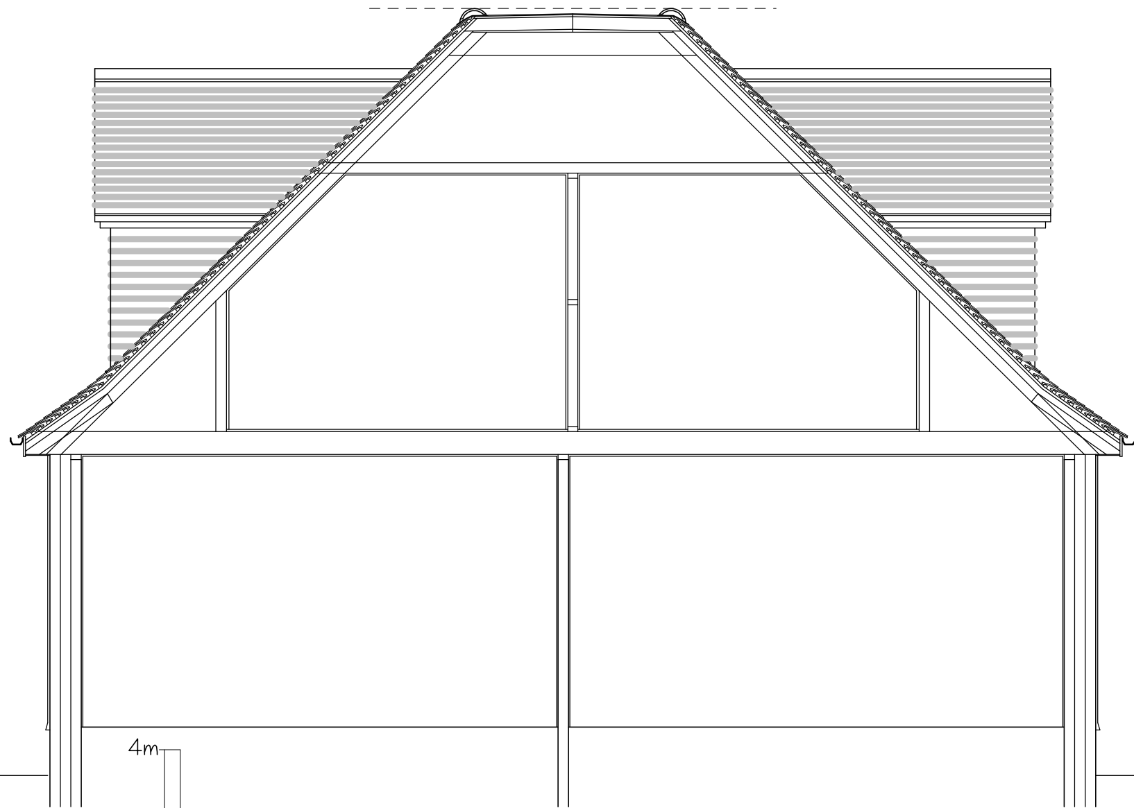
SECTION THROUGH EXTENSION - 1:50
