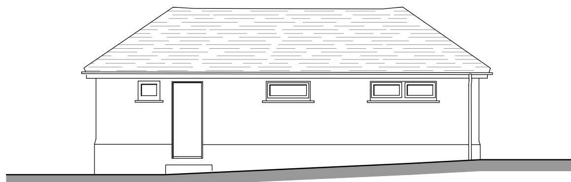
EXISTING REAR ELEVATION (NE)
