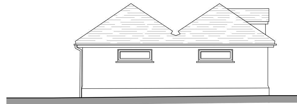
EXISTING SIDE ELEVATION (NW)
