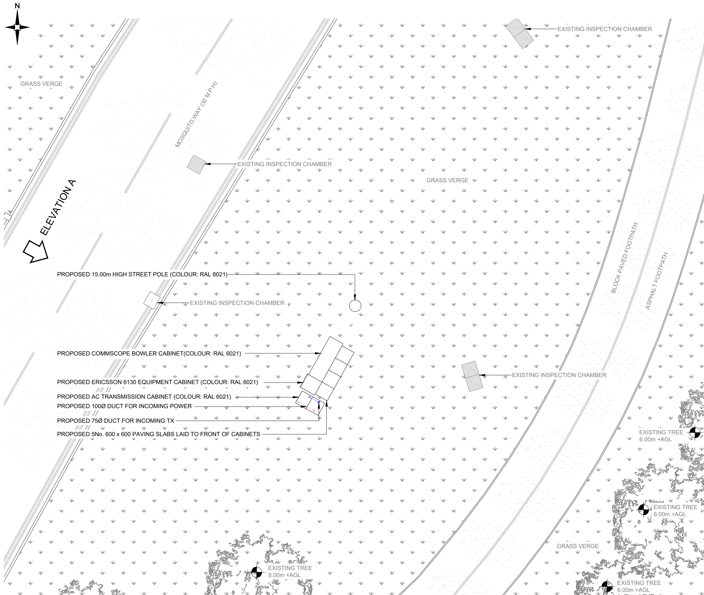
PROPOSED SITE PLAN 1:100
