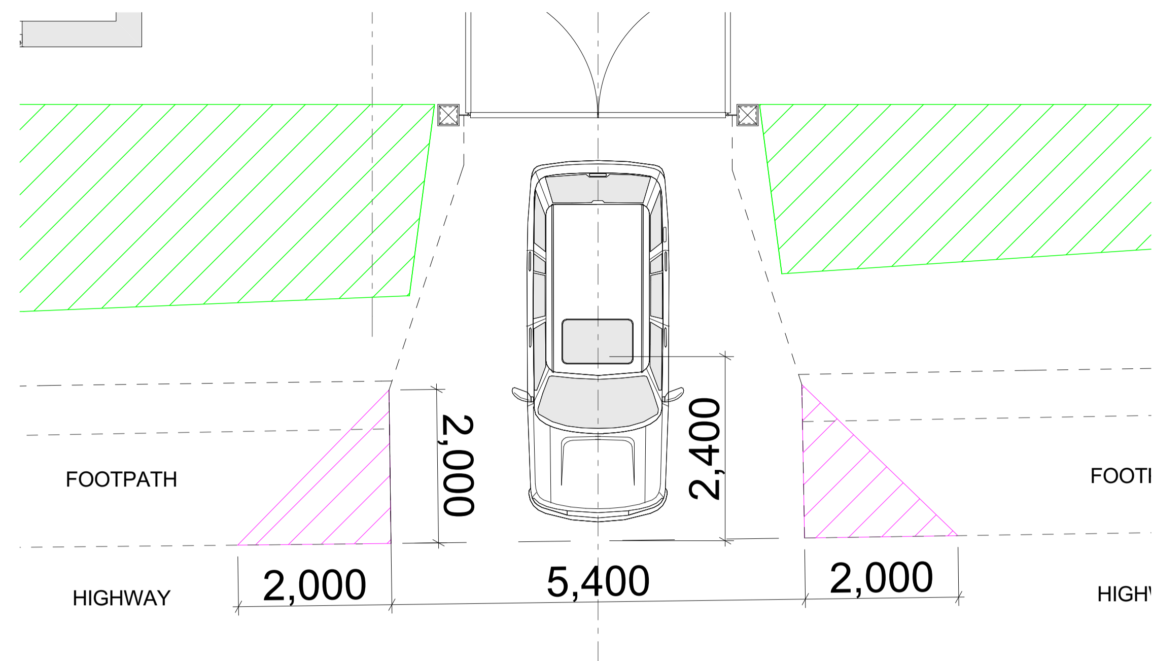
2M X 2M X 0.6M HIGH PEDESTRIAN VISABILITY SPLAY 1:50
