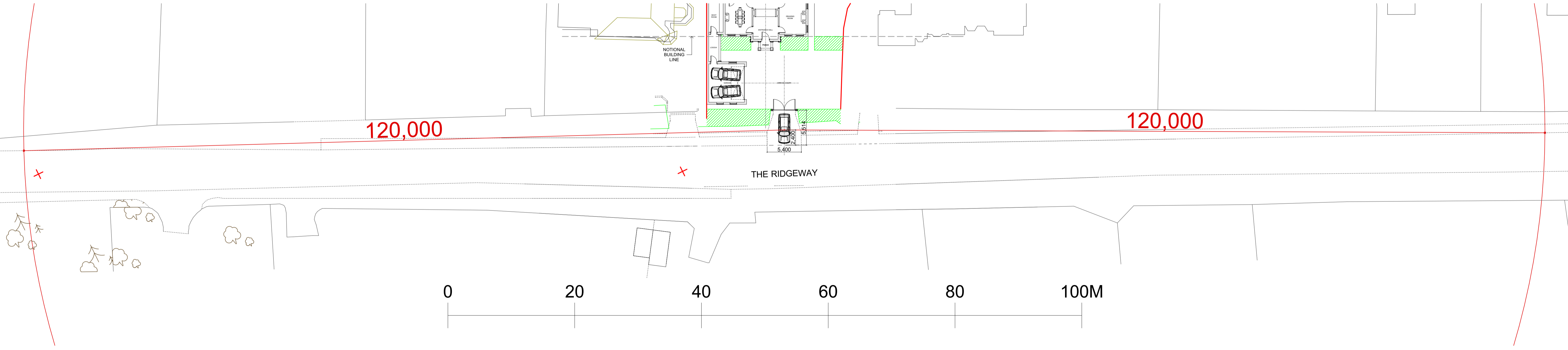
2.4M X 120M VEHICULAR VISABILITY SPLAY 1:300
