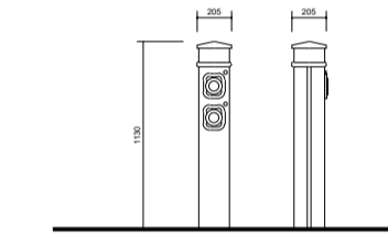
EV pedestal (2 sockets)
