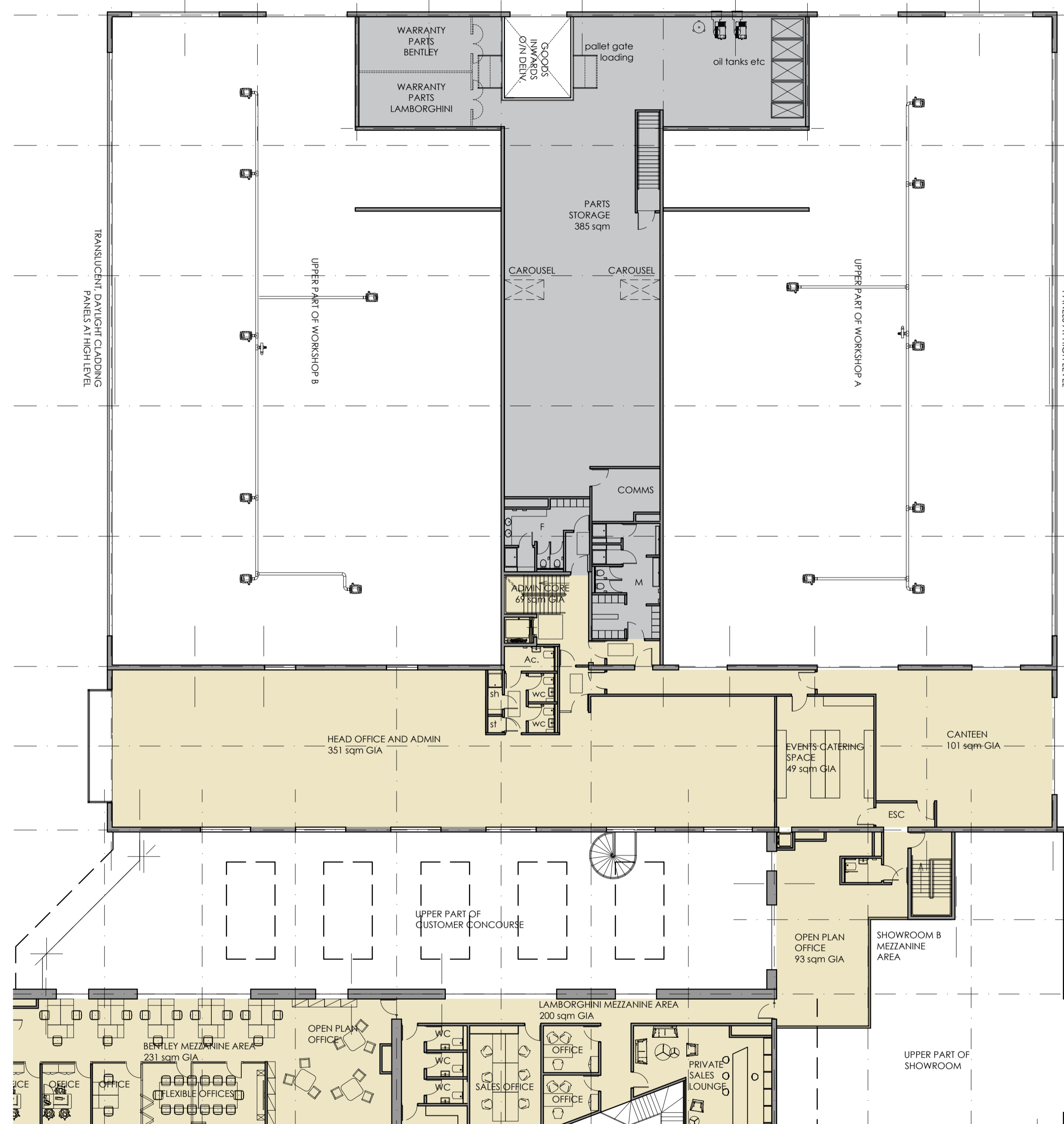
FIRST FLOOR 1:200
