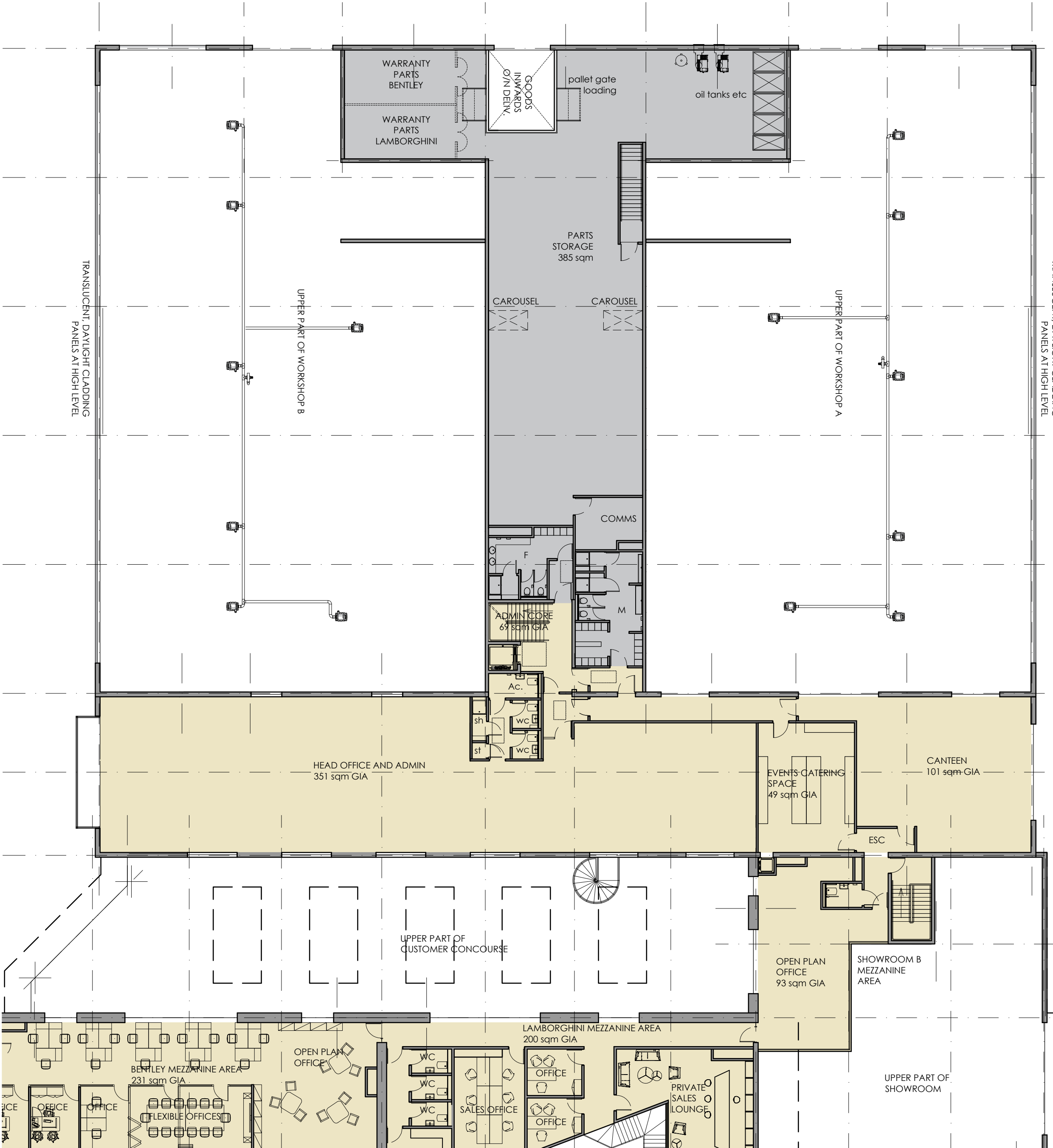
FIRST FLOOR 1:200
