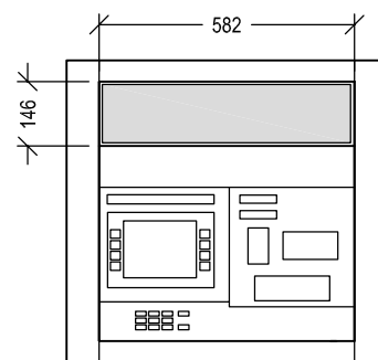
ELEVATION ON FASCIA Scale 1:20
