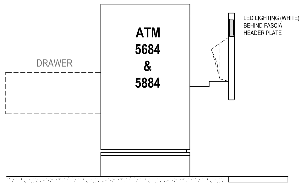
TYPICAL SECTION Scale 1:20
