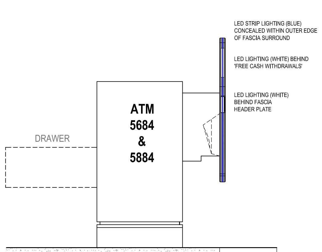
TYPICAL SECTION Scale 1:20
