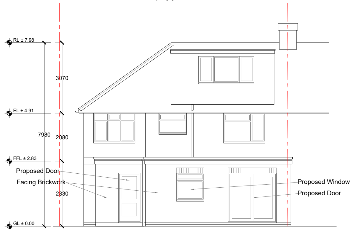
Proposed Front Elevation (North)
