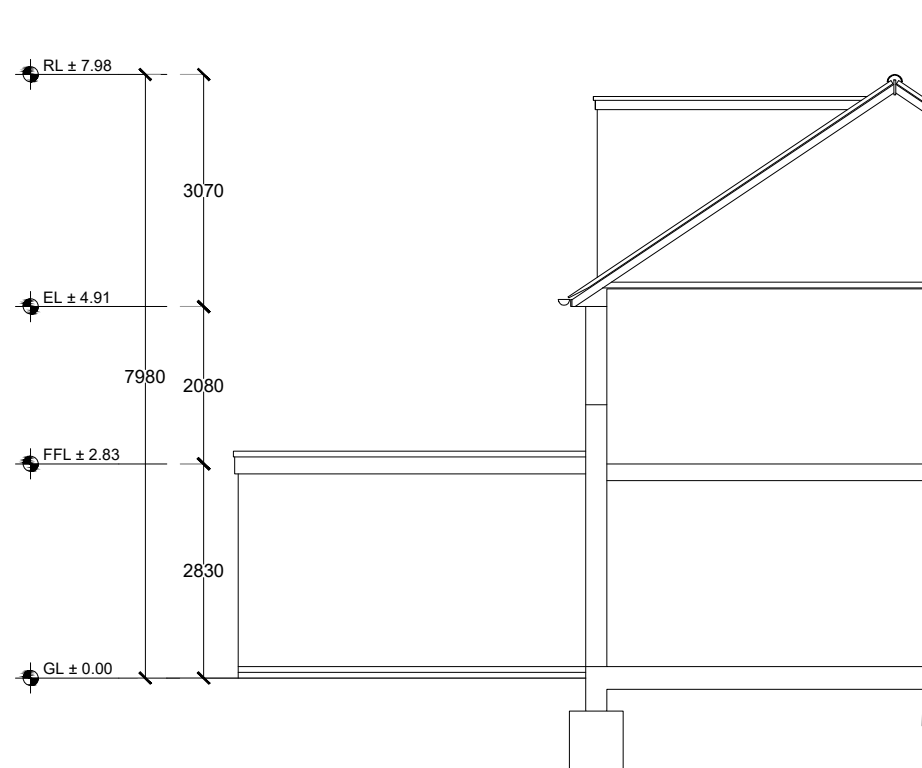
Proposed Side Elevation (Section A-A)
