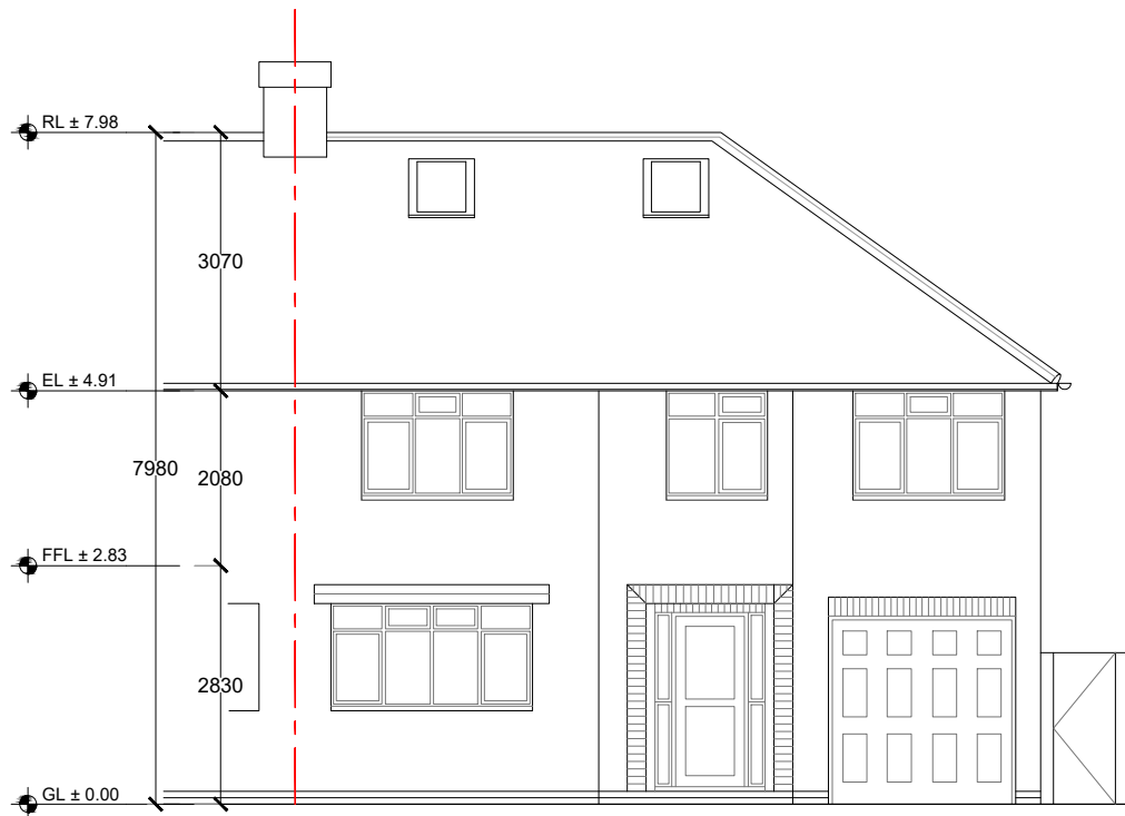
Existing Front Elevation (North)
