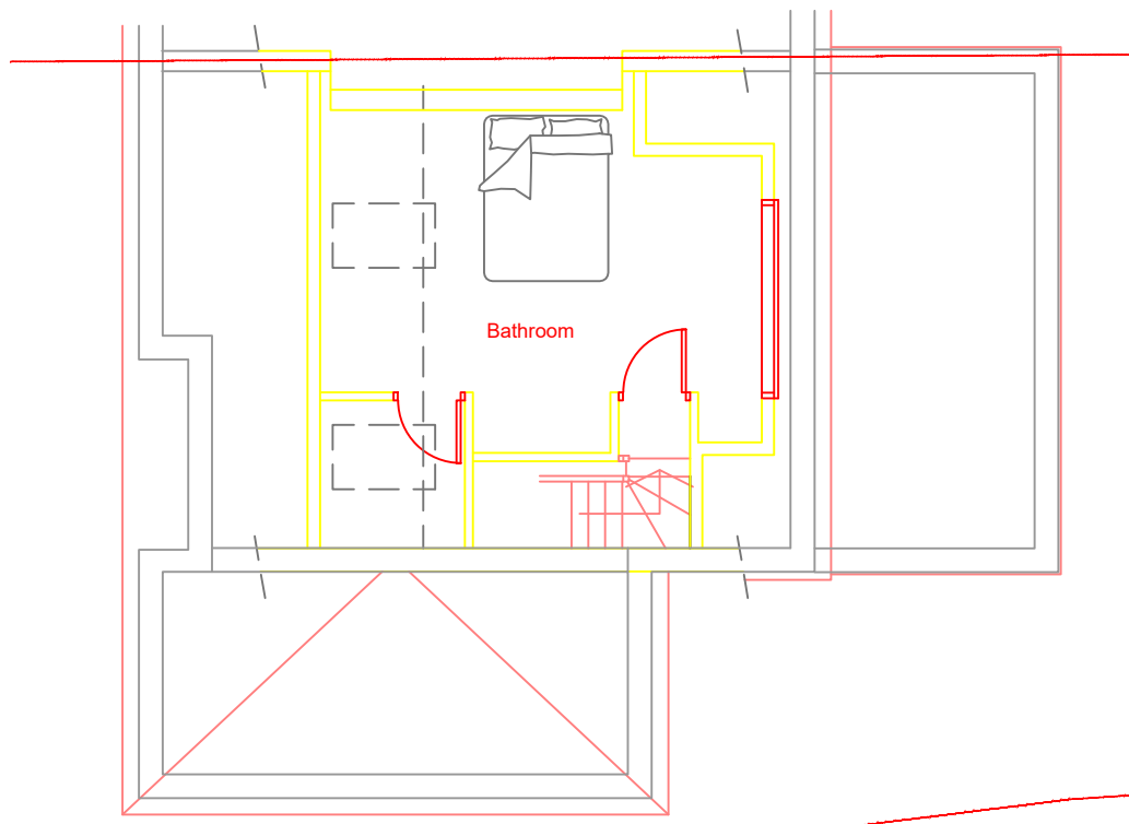
Existing Second Floor Plan
