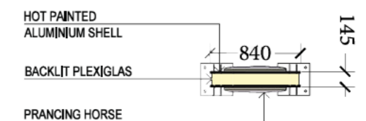
TOP PLAN SCALE 1:50
