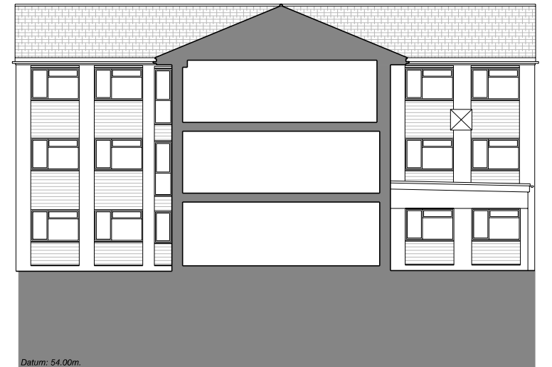
05 Elevation 8 1:200@A3
