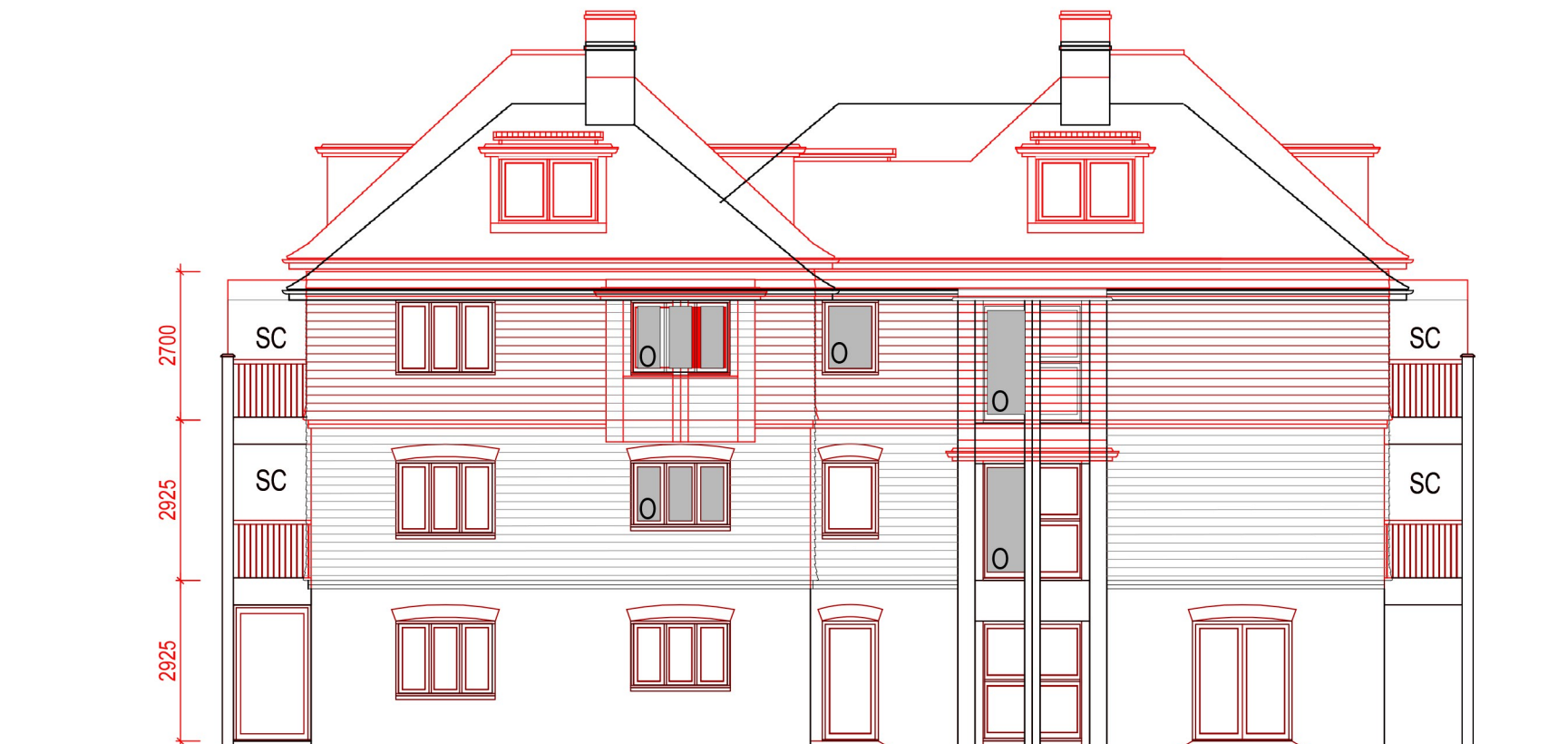
SOUTH ELEVATION (New)
