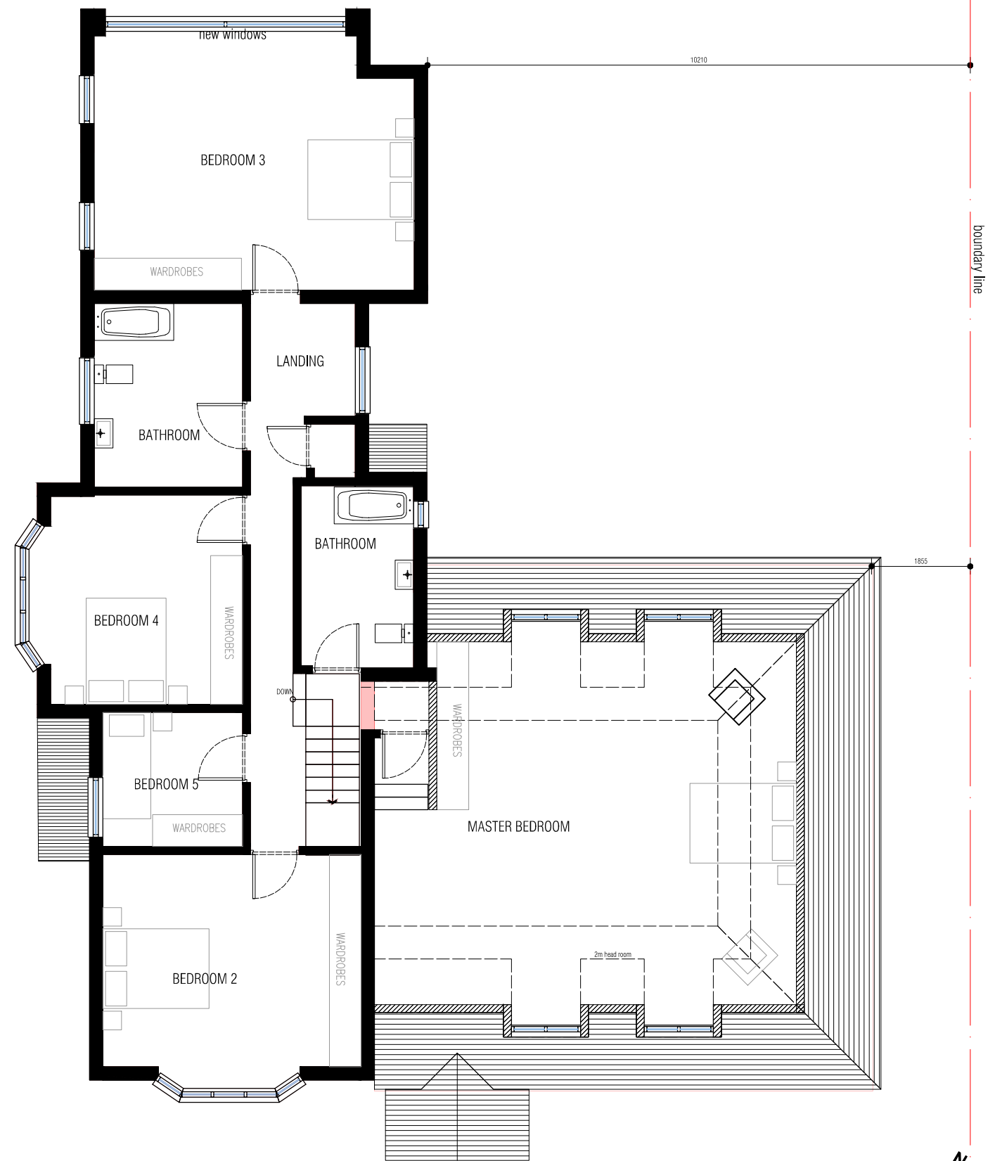
[02] PROPOSED FIRST FLOOR FLOOR PLAN
