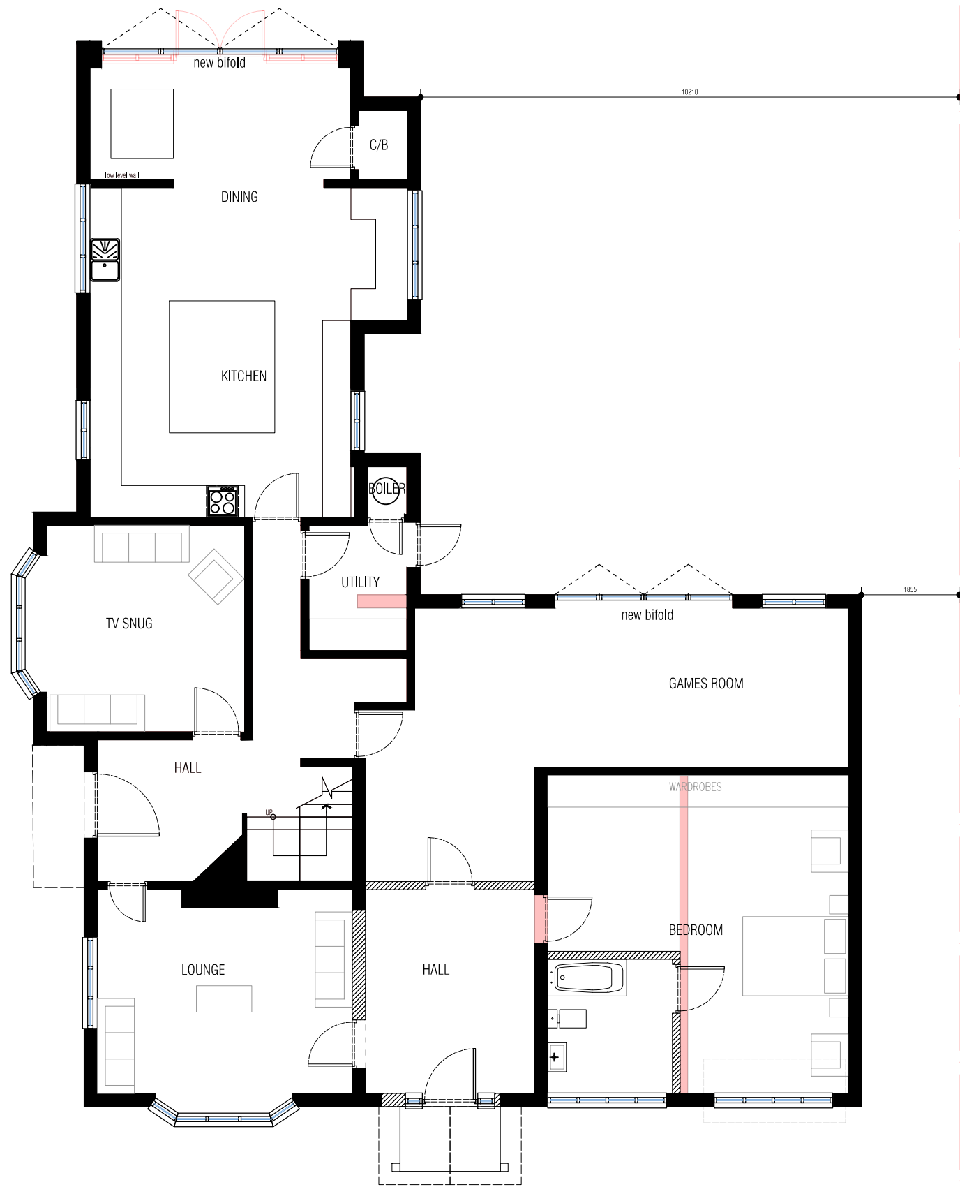
[01] PROPOSED GROUND FLOOR PLAN
