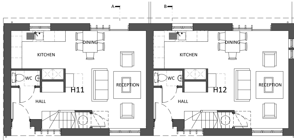
H11 GROUND FLOOR
