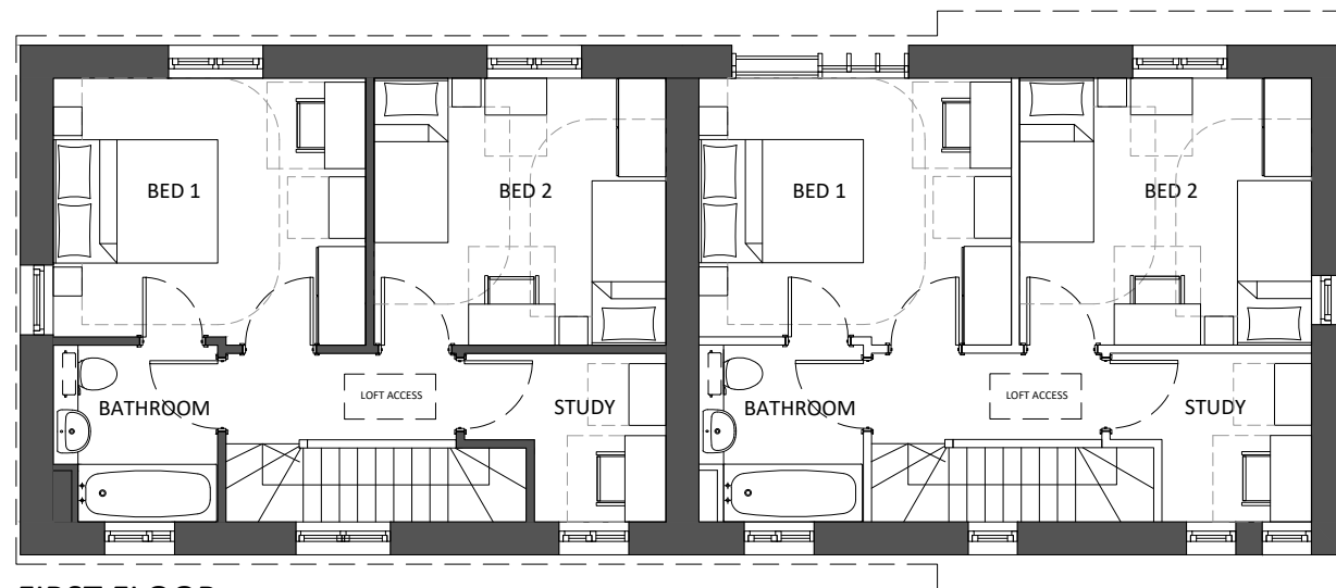
FIRST FLOOR
