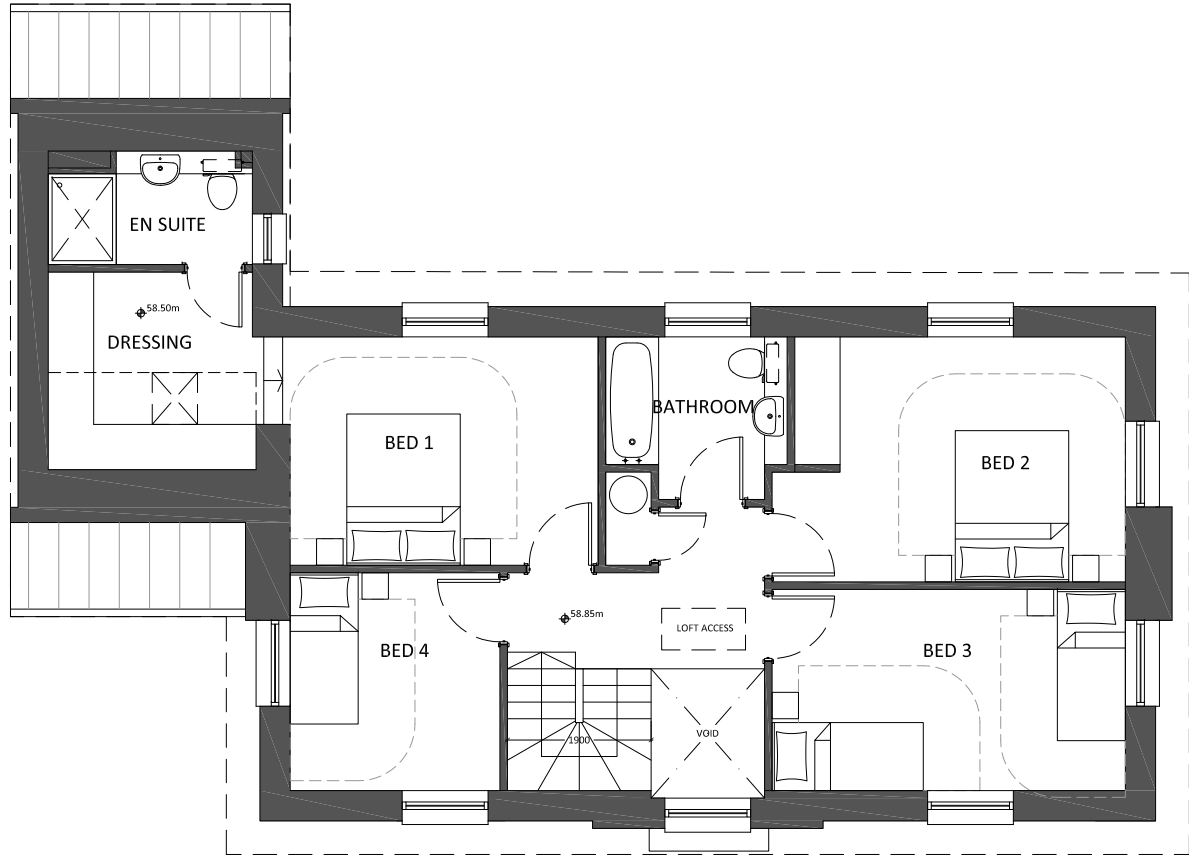
FIRST FLOOR
