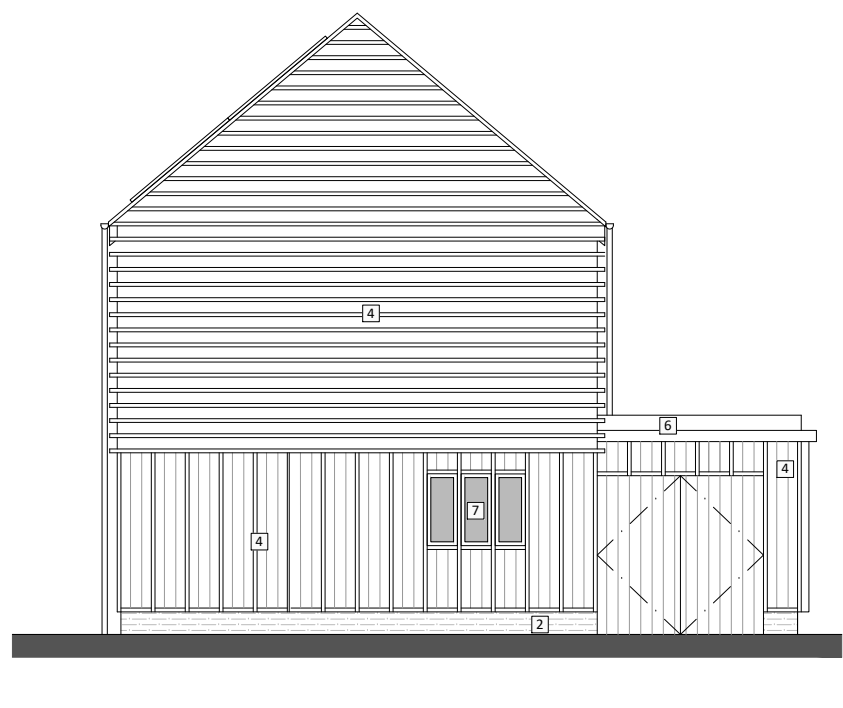
RH SIDE (NE) ELEVATION
