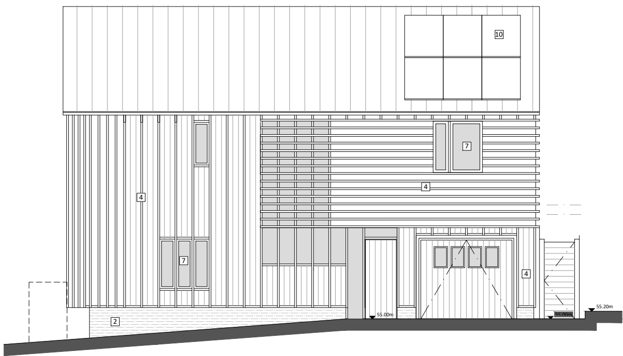
FRONT (SE) ELEVATION
